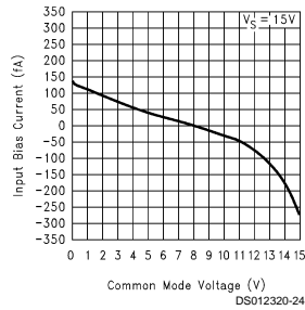
Input Current vs Common-Mode Voltage
