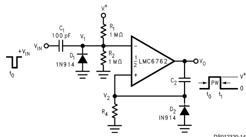
FIGURE 6. One-Shot Multivibrator
