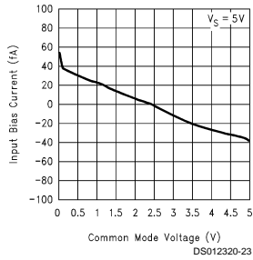
Input Current vs Common-Mode Voltage
