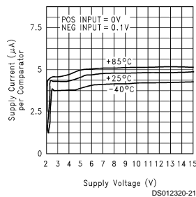
Supply Current vs Supply Voltage (Output Low)
