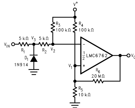
FIGURE 8. Zero Crossing Detector
