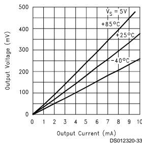
Output Voltage vs Output Current (Sinking)
