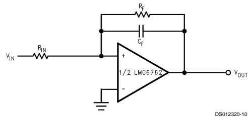
FIGURE 5. Canceling the Effect of Input Capacitance
