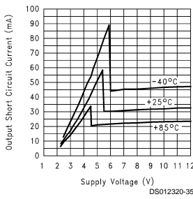
Output Short Circuit Current vs Supply Voltage (Sourcing)
