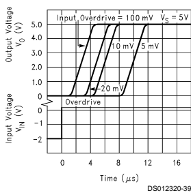
Response Time for Overdrive ( t_{PLH} )
