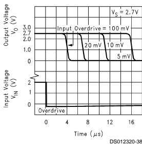
Response Time for Overdrive ( t_{PHL} )
