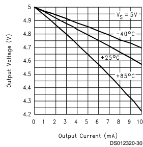
Output Voltage vs Output Current (Sourcing)
