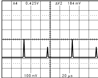
FIGURE 4. Measurement of the Shoot-Through Current
