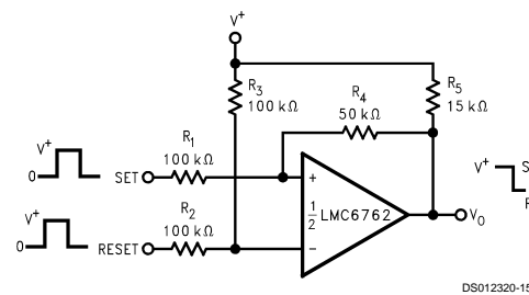
FIGURE 7. Bi-Stable Multivibrator
