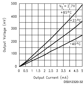
Output Voltage vs Output Current (Sinking)
