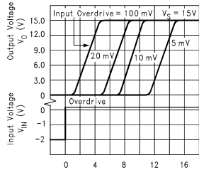
Response Time for Overdrive ( t_{PLH} )
