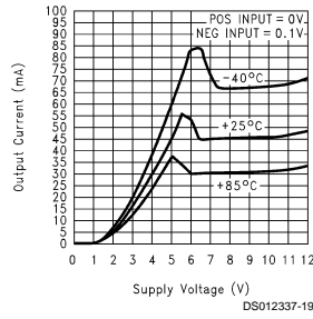
Output Sinking Current vs Supply Voltage
