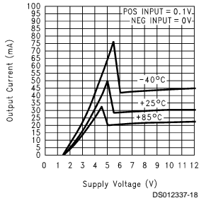
Output Sourcing Current vs Supply Voltage
