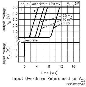
Response Time for Various Input Overdrives -t_{PLH}
