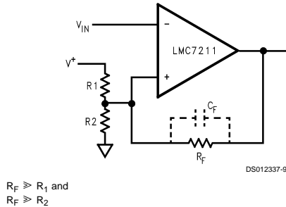
FIGURE 4. Positive Feedback for Hysteresis
