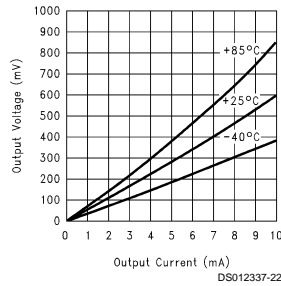
Output Sourcing Current vs Output Voltage @ 15V
