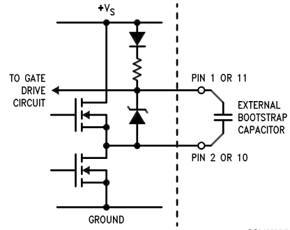
FIGURE 6. Bootstrap Circuitry
