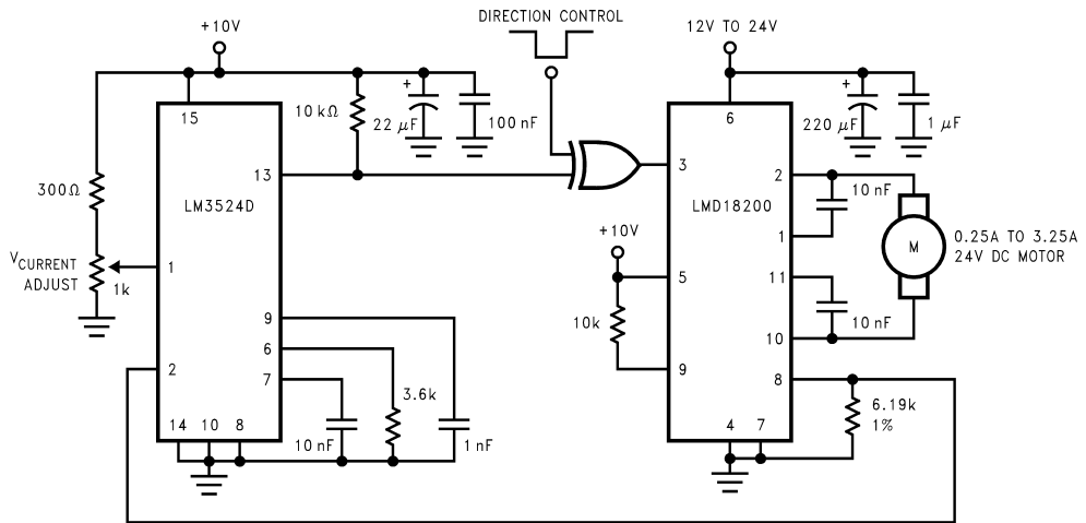
FIGURE 9. Locked Anti-Phase Control Regulates Torque
