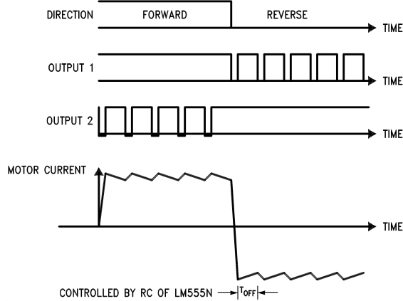
FIGURE 8. Switching Waveforms
