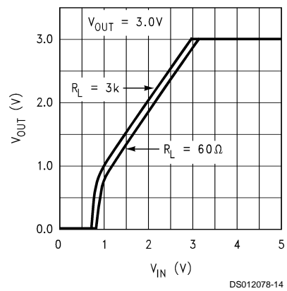
Dropout Characteristics
