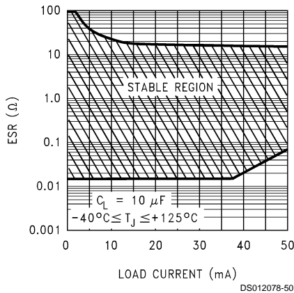
FIGURE 3. 10 μF ESR Range
