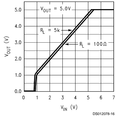
Dropout Characteristics
