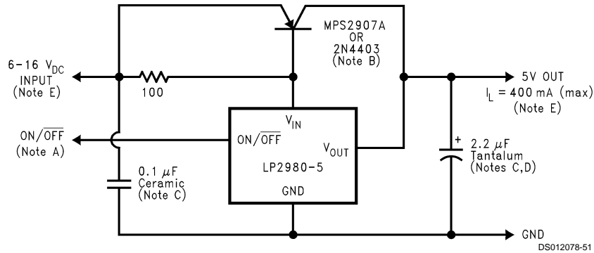
FIGURE 5. 5V/400mA Regulator
