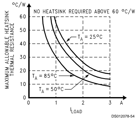
FIGURE 8. Heatsink Thermal Resistance Requirements for Figure 7
