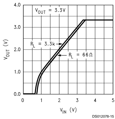
Dropout Characteristics
