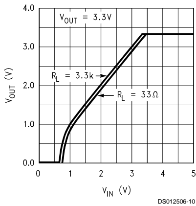
Dropout Characteristics
