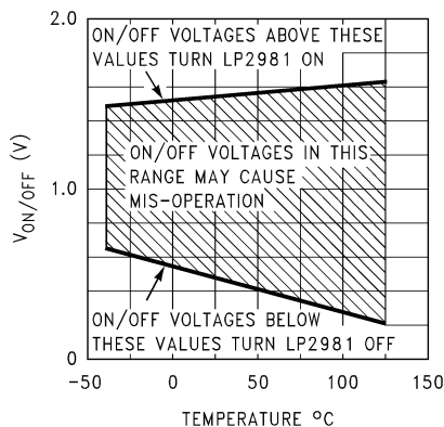
ON/OFF Threshold vs Temperature
