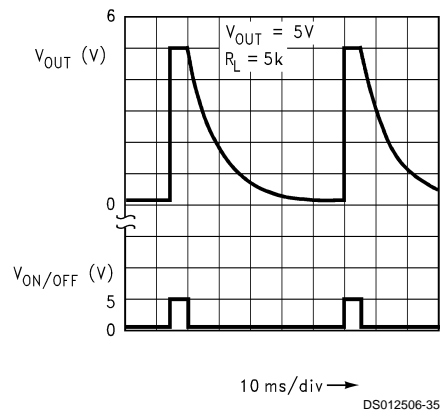
Turn-Off Waveform
