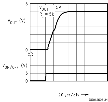
Turn-On Waveform
