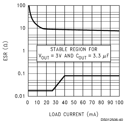
FIGURE 3. 3V/3.3 \mu F ESR Curves
