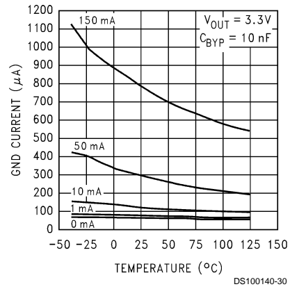
GND Pin Current vs Temperature
