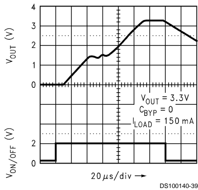
Turn-On Time
