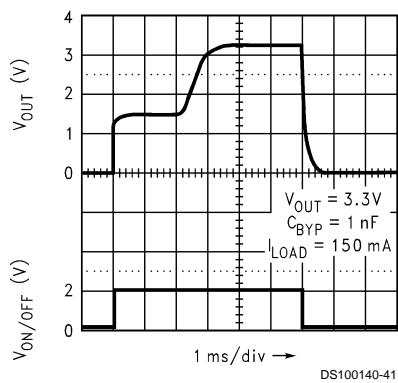
Turn-On Time
