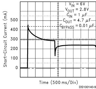
Short-Circuit Current
