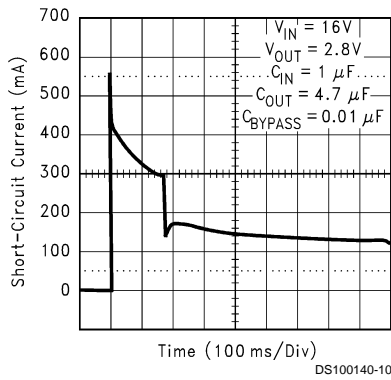
Short-Circuit Current
