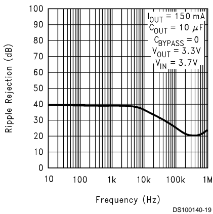
Ripple Rejection
