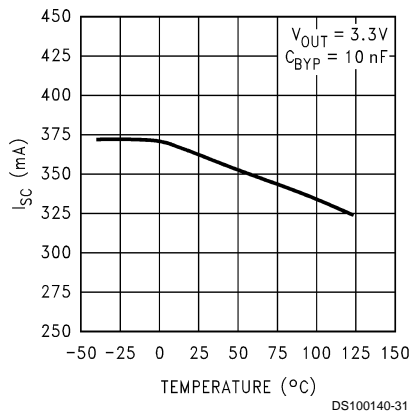
Instantaneous Short Circuit Current
