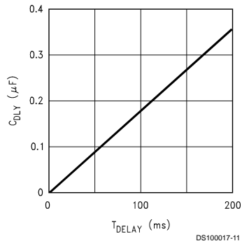
Plot of C_{DLY} vs T_{DELAY}
