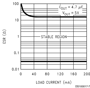
ESR Curves For 5V Output
