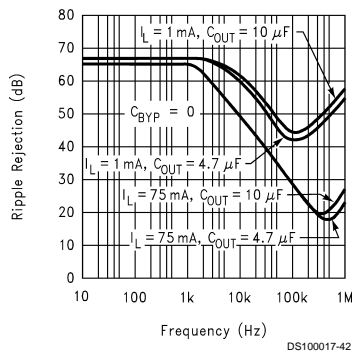
Ripple Rejection (LP2987)
