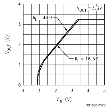
Dropout Characteristics
