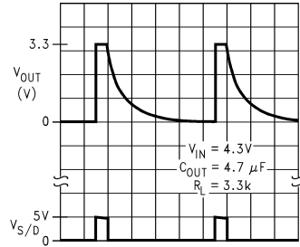
Turn-On Waveform
