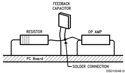
FIGURE 6. Air Wiring
