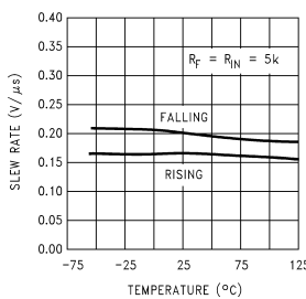
Inverting Slew Rate vs Temperature
