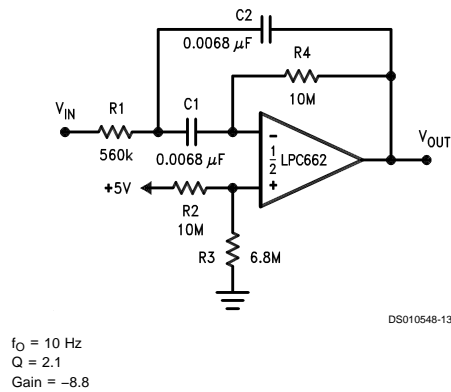
10 Hz Bandpass Filter
