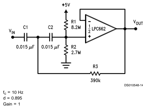
10 Hz High-Pass Filter (2 dB Dip)
