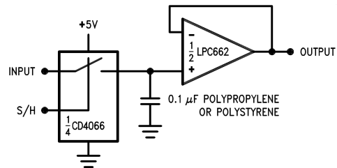
Low-Leakage Sample-and-Hold
