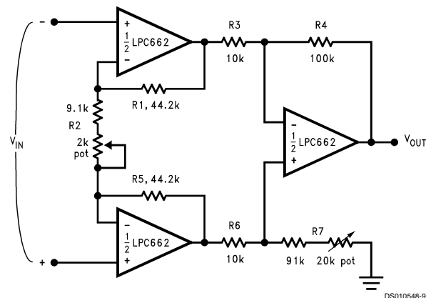
Instrumentation Amplifier
