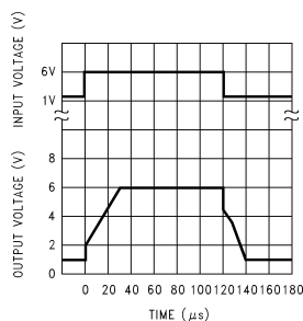
Large-Signal Pulse Non-Inverting Response ( A_V = +1 )
