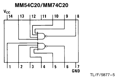
Top View Order Number MM54C20 or MM74C20
