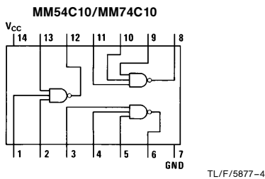
Top View Order Number MM54C10 or MM74C10
