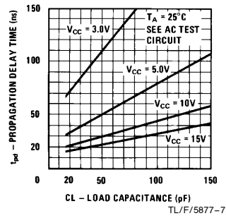
Propagation Delay Time vs Load Capacitance MM54C20/MM74C20
