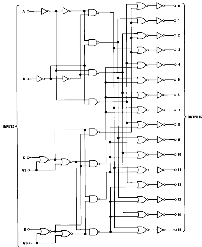
TL/F/5893-1
