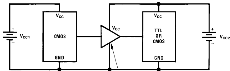
CMOS to TTL or CMOS at a Lower V_{CC}
