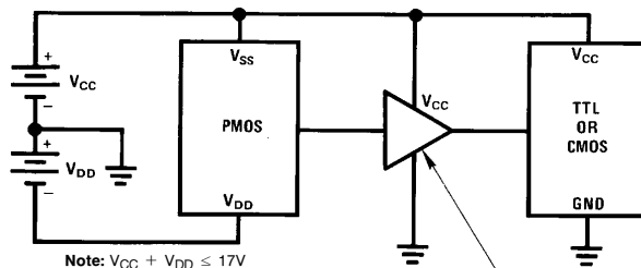
PMOS to CMOS or TTL Interface
