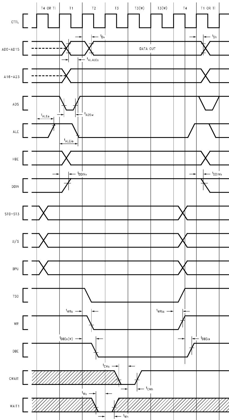
FIGURE 4-5. Write Cycle
