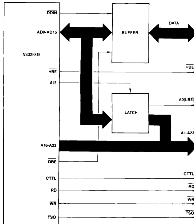
FIGURE 3-20. Bus Connections
