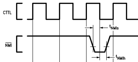
FIGURE 4-17. \overline{\text{NMI}} Signal Timing
