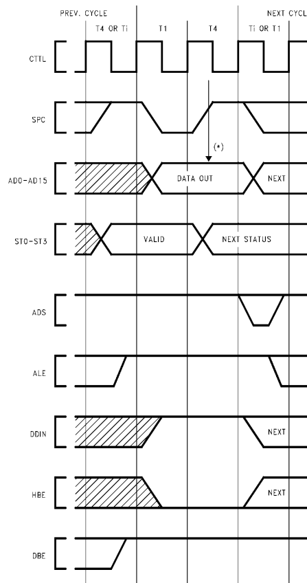
FIGURE 3-26. Slave Processor Write Cycle
