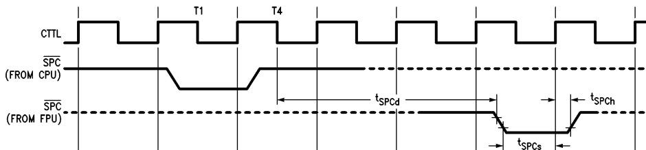
FIGURE 4-12. SPC Timing
