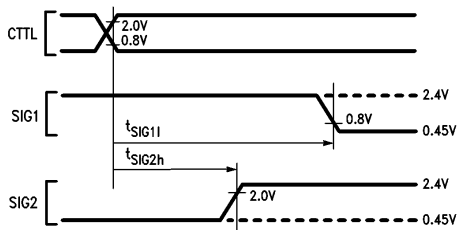
FIGURE 4-2. Output Signals Specification Standard TL/EE/10818-40
