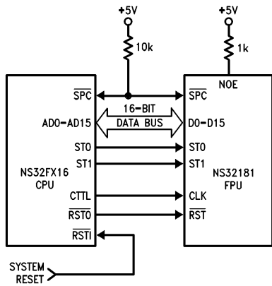
TL/EE/10818-33 FIGURE 3-27. NS32FX16 and FPU Interconnections
