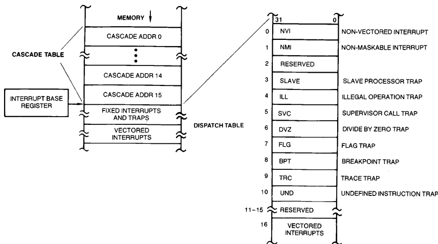
FIGURE 3-4. Interrupt Dispatch and Cascade Tables
