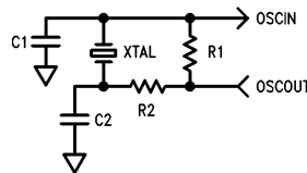
FIGURE 3-15. Crystal Interconnections—30 MHz
