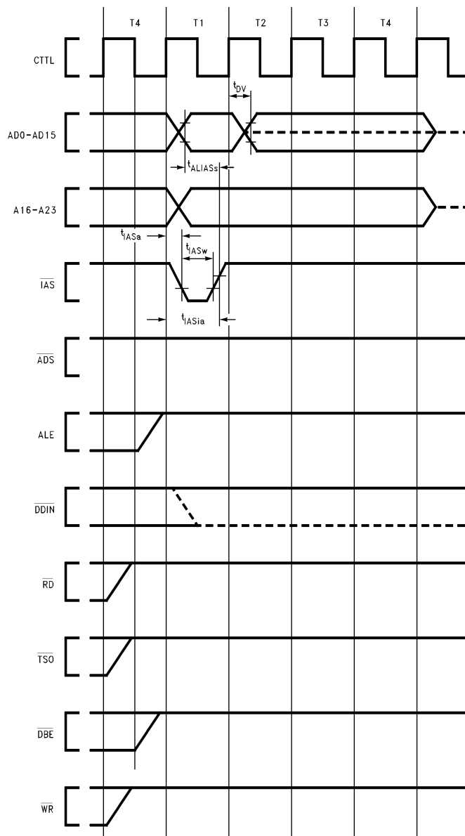
FIGURE 4-6. Special Bus Cycle
