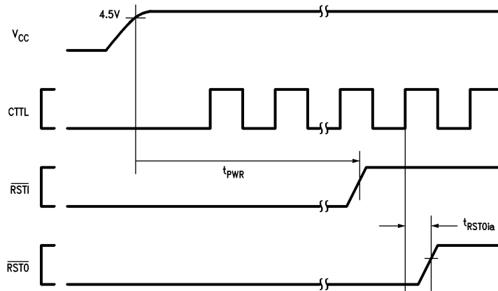
FIGURE 4-18. Power-On Reset
