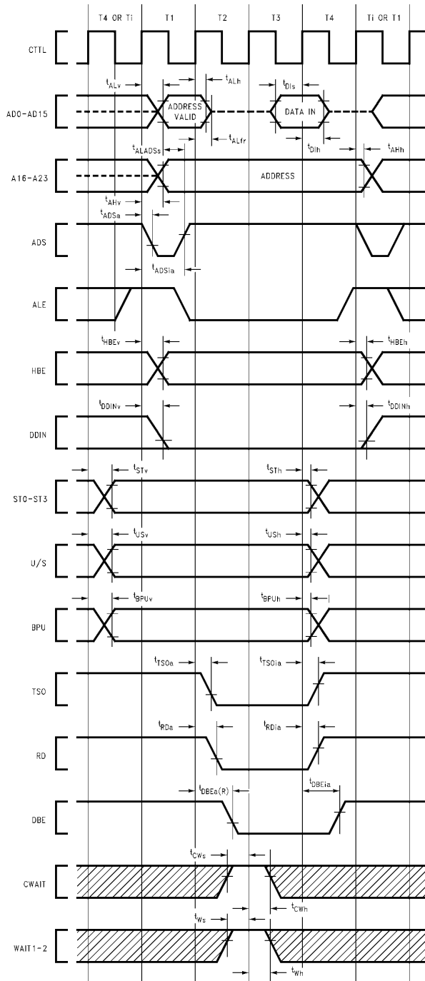
FIGURE 4-4. Read Cycle
