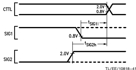
FIGURE 4-3. Input Signals Specification Standard TL/EE/10818-41
