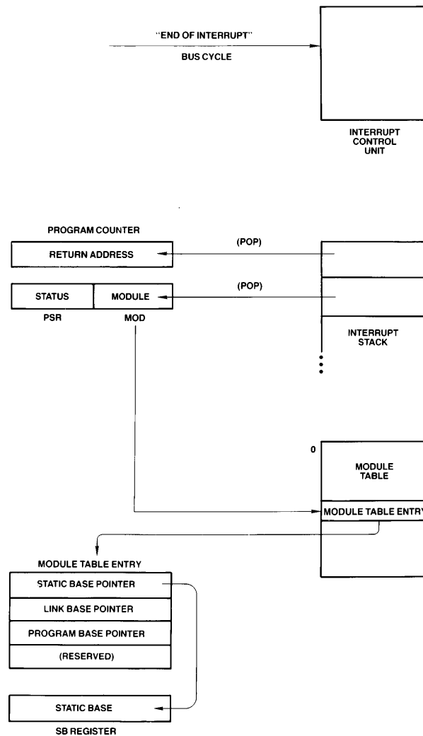
FIGURE 3-7. Return from Interrupt (RETI) Instruction Flow
