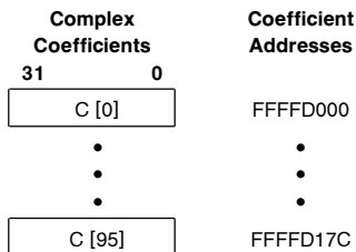
FIGURE 2-8. On-Chip RAM Array Address Map
