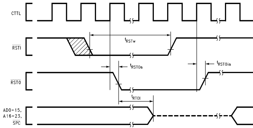
FIGURE 4-19. Non-Power-On Reset
