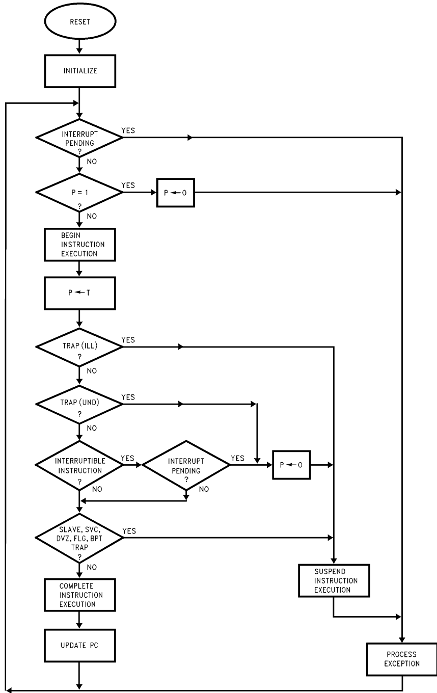
FIGURE 3-10. Exception Processing Flowchart
