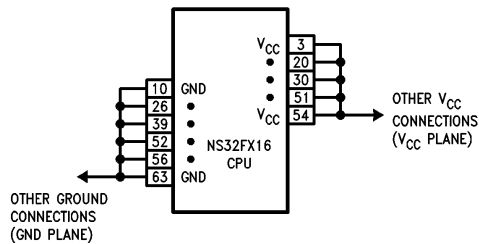
FIGURE 3-14. Power and Ground Connections
