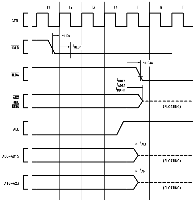
FIGURE 4-7. \overline{\text{HOLD}} Acknowledge Timing (Bus Initially Not Idle)
