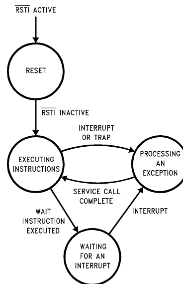
FIGURE 3-1. Operating States
