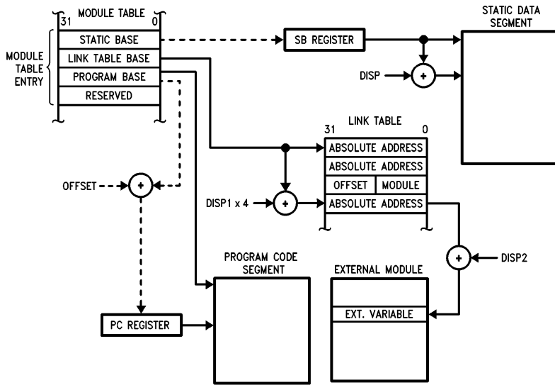
FIGURE 2-10. NS32FX16 Run-Time Environment
