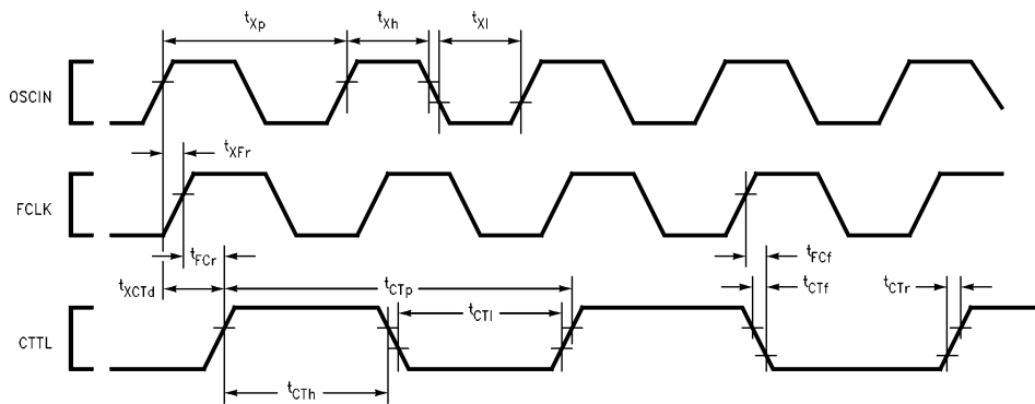
FIGURE 4-15. Clock Waveforms
