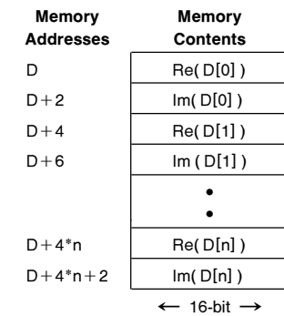
FIGURE 3-13. Memory Organization of a Complex Vector
