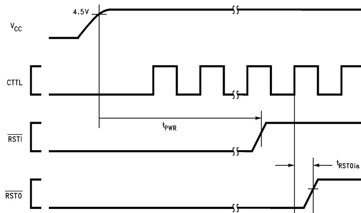
FIGURE 4-18. Power-On Reset
