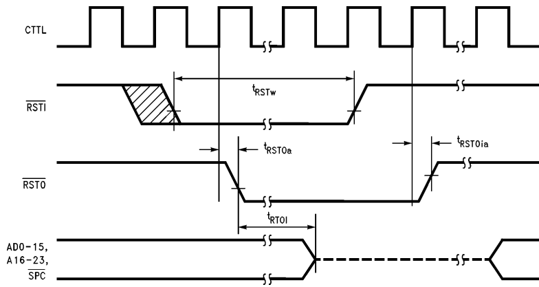
FIGURE 4-19. Non-Power-On Reset
