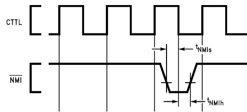
FIGURE 4-17. NMI Signal Timing
