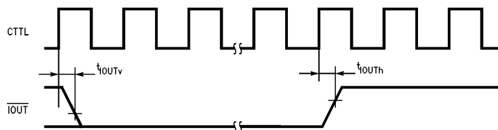
FIGURE 4-20. Interrupt Out
