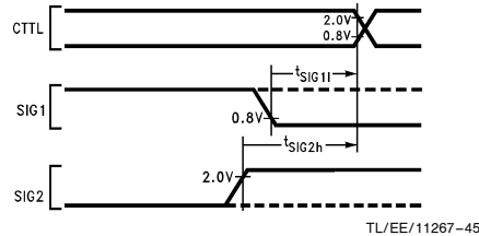
FIGURE 4-3a. Input Signals Specification Standard
