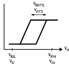
FIGURE 4-3b. \overline{RSTI} , \overline{INT} , \overline{NMI} Hysteresis
