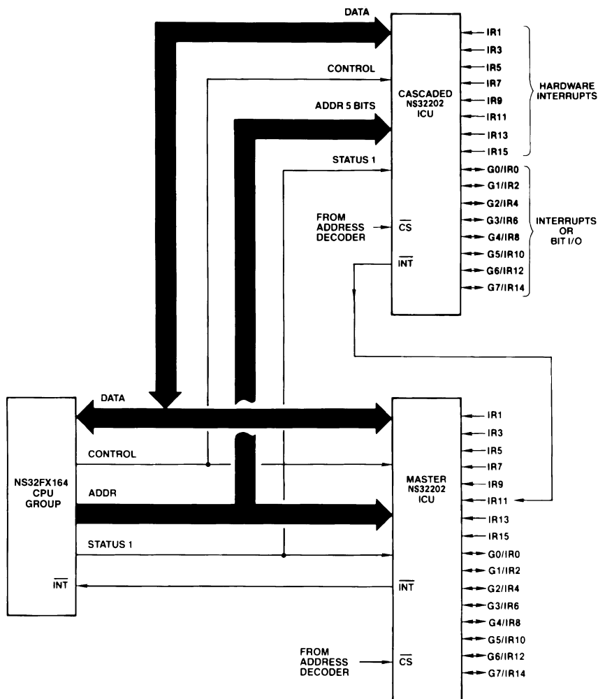
FIGURE 3-10. Cascaded Interrupt Control Unit Connections
