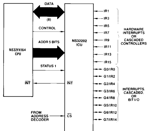
FIGURE 3-9. Interrupt Control Unit Connections (16 Levels)
