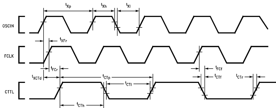
FIGURE 4-15. Clock Waveforms
