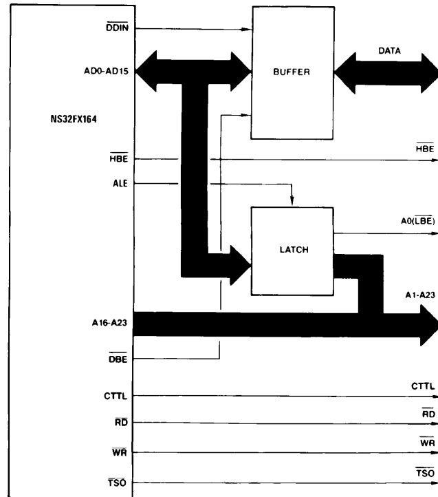
FIGURE 3-20. Bus Connections
