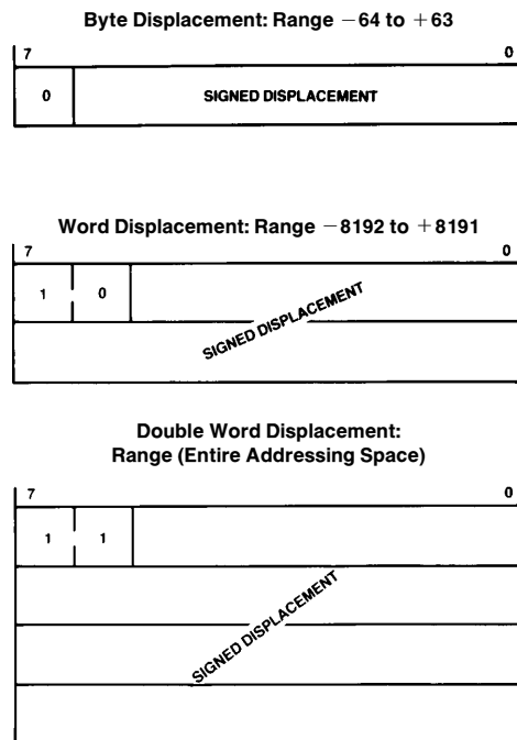
FIGURE 2-19. Displacement Encodings
