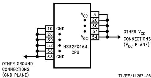
FIGURE 3-14. Power and Ground Connections
