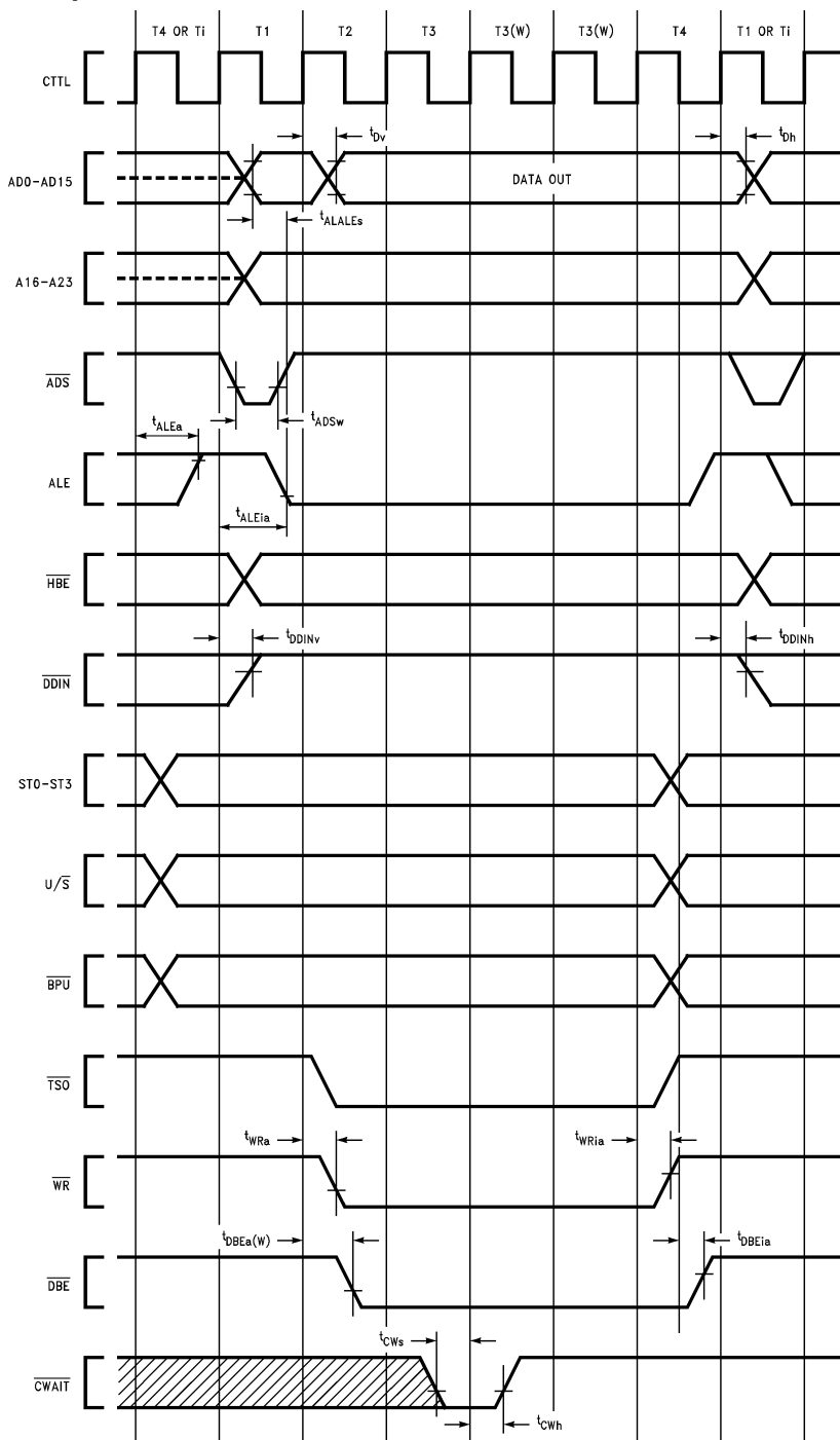
FIGURE 4-5. Write Cycle
