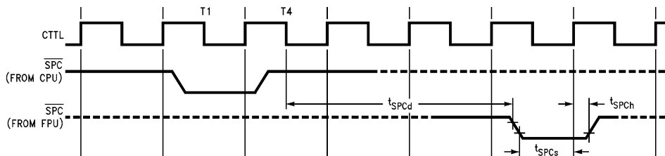
FIGURE 4-12. SPC Timing
