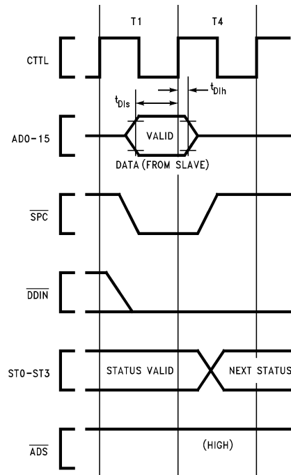
FIGURE 4-11. Slave Processor Read Timing
