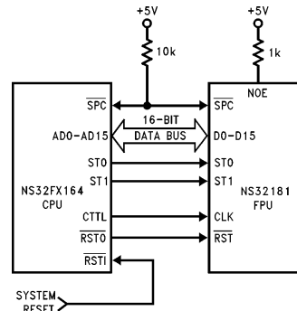
FIGURE 3-27. NS32FX164 and FPU Interconnections
