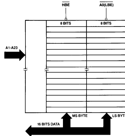
FIGURE 3-28. Memory Interface
