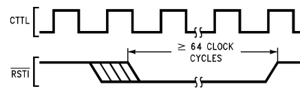
FIGURE 3-19. General Reset Timing
