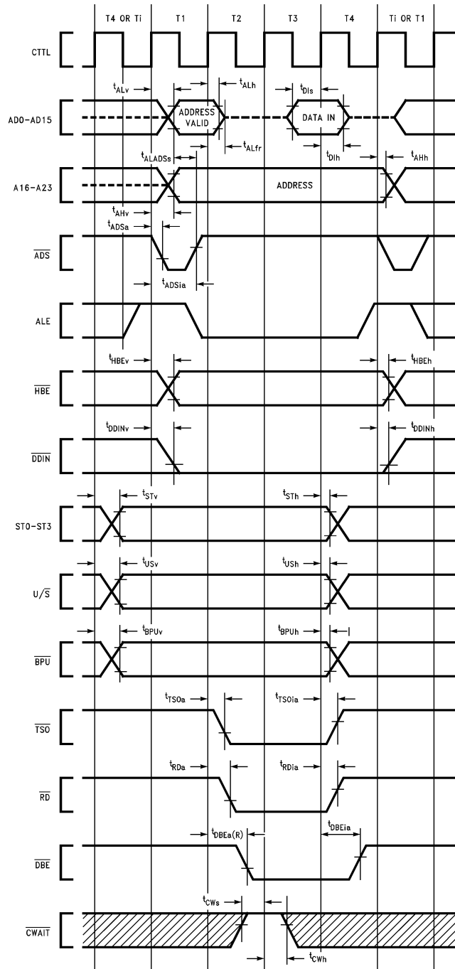
FIGURE 4-4. Read Cycle
