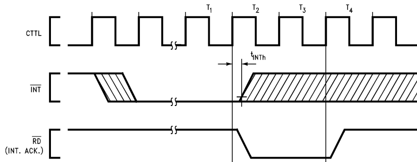
FIGURE 4-16. INT Signal Timing
