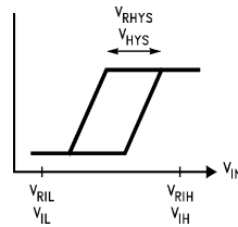
FIGURE 4-3b. \overline{RSTI} , \overline{INT} , \overline{NMI} Hysteresis
