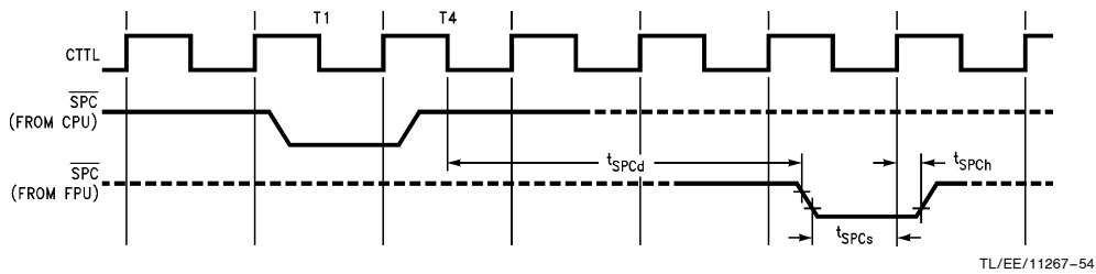
FIGURE 4-12. SPC Timing
