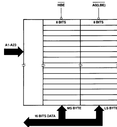
FIGURE 3-28. Memory Interface
