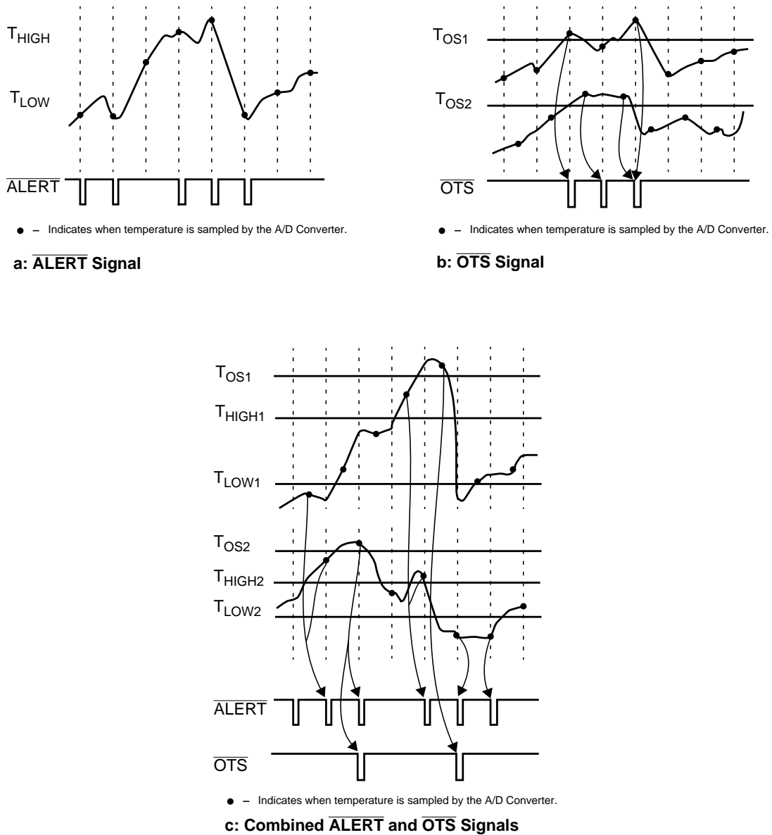
Figure 43. \overline{\text{OTS}} and \overline{\text{ALERT}} Temperature Response Diagrams
