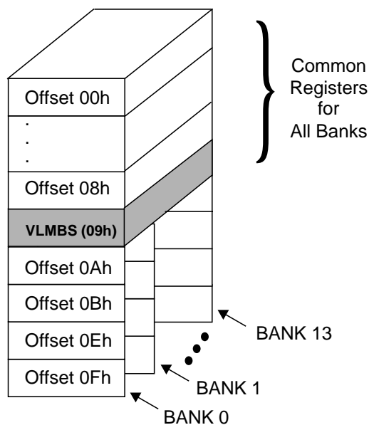
Figure 38. Register Bank Architecture
