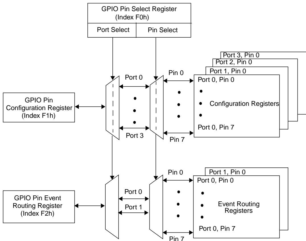
Figure 6. Organization of GPIO Pin Registers
