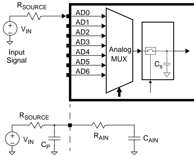
Figure 39. Analog Input Schematic Diagram and Equivalent R-C Circuit
