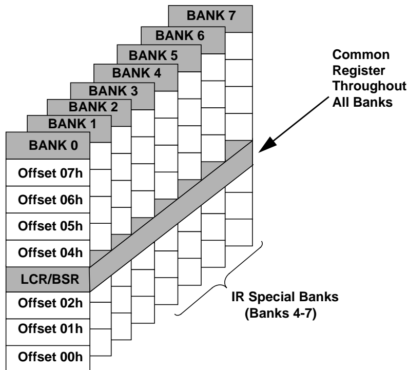
Figure 48. SP2 Register Bank Architecture
