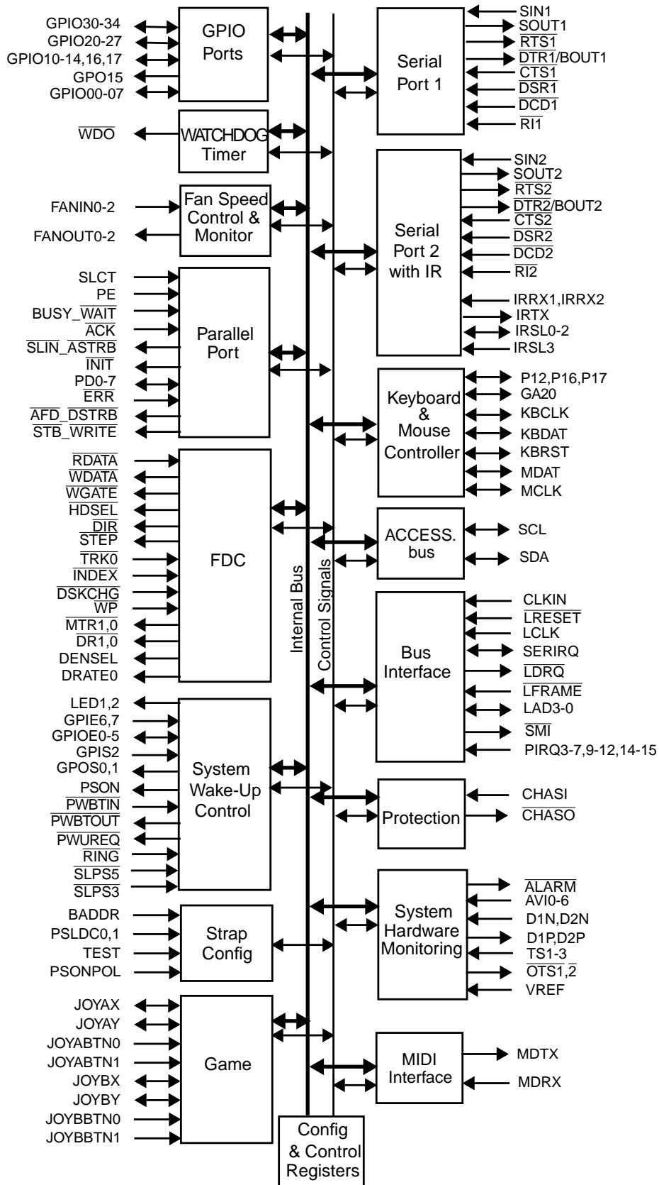
Figure 1. PC87366 Detailed Block Diagram
