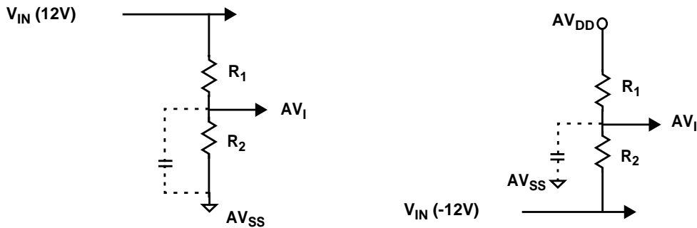
Figure 40. Measurement of Positive and Negative Voltages
