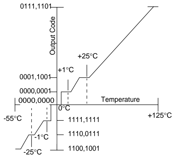
Figure 44. Temperature-to-Digital Transfer Function (Non-linear scale for clarity)
