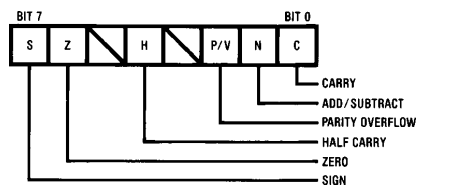
FIGURE 5. Flag Register
