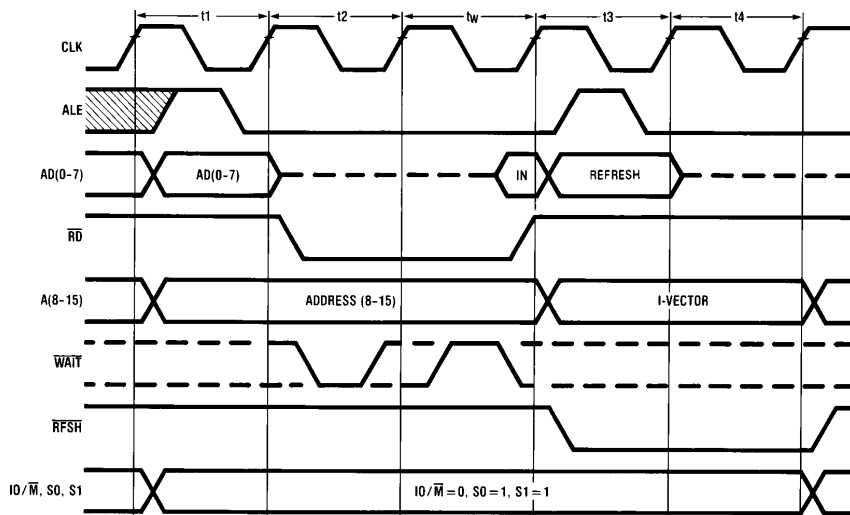
FIGURE 9b. Opcode Fetch Cycles with \overline{WAIT} States
