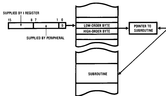
FIGURE 17. Interrupt Mode 2
