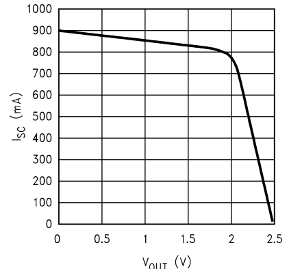
Short Circuit Current vs V_OUT
