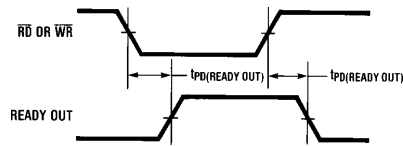
FIGURE 4. Ready Out
