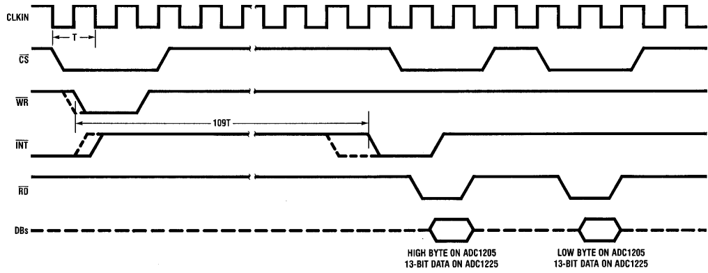
FIGURE 3. Timing Diagram
