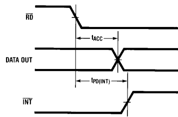
FIGURE 5. Data Out
