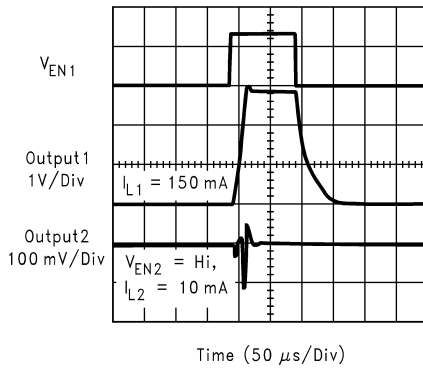
Enable Response ( V_{IN} = V_{OUT} + 0.2V )
