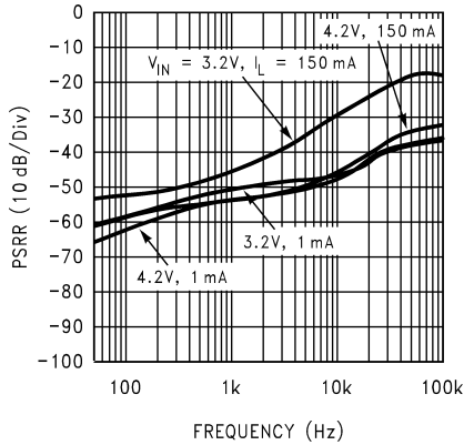
Power Supply Rejection Ratio ( C_{BP} = 0.001\mu\text{F} )
