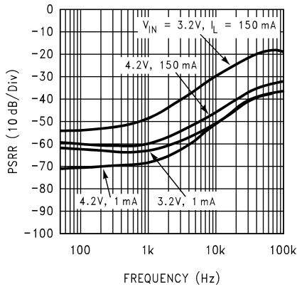
Power Supply Rejection Ratio ( C_{BP} = 0.1\mu\text{F} )
