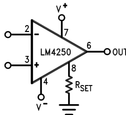
R SET Connected to Ground
