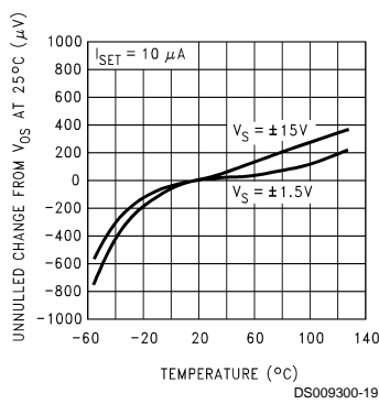
Unnull'd Input Offset Voltage Change vs Temperature
