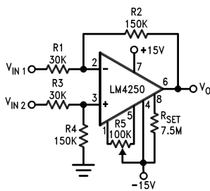
X5 Difference Amplifier
