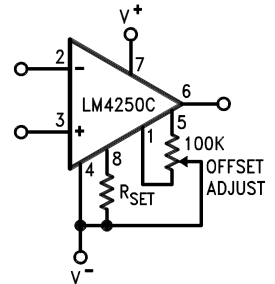
Offset Null Circuit
