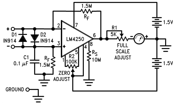
Floating Input Meter Amplifier 100 nA full Scale
