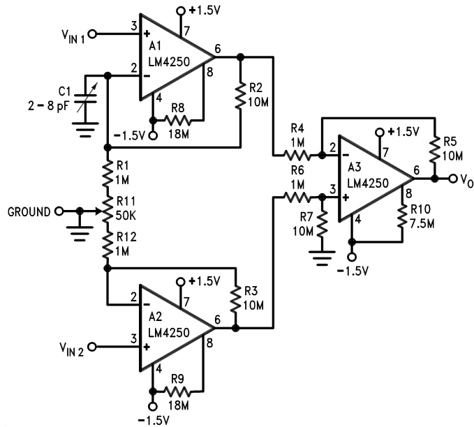
X100 Instrumentation Amplifier 10 \mu W
