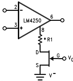
FET Current Sourcing Biasing
