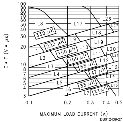
FIGURE 7. LM2594/LM2594HV-ADJ
