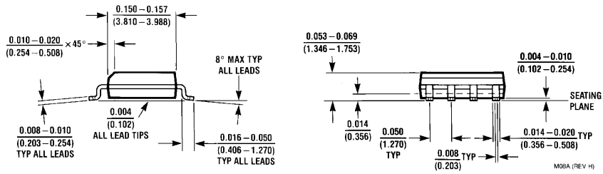
8-Lead (0.150" Wide) Molded Small Outline Package, Order Number LM2594M-3.3, LM2594M-5.0, LM2594M-12 or LM2594M-ADJ JEDEC NS Package Number M08A
