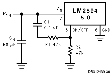
FIGURE 21. Delayed Startup
