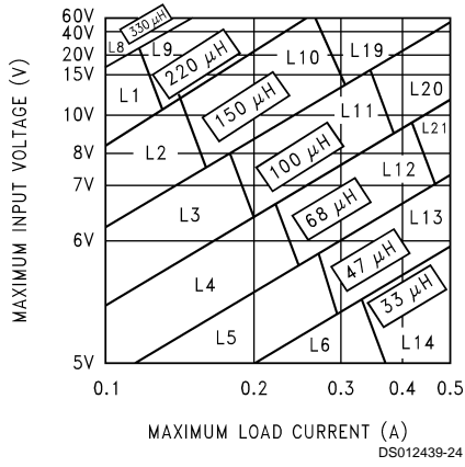
FIGURE 4. LM2594/LM2594HV-3.3
