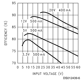
Efficiency
