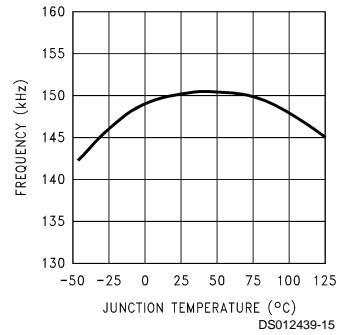
Switching Frequency
