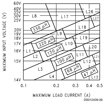
FIGURE 6. LM2594/LM2594HV-12
