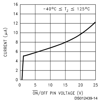
ON /OFF Pin Current (Sinking)
