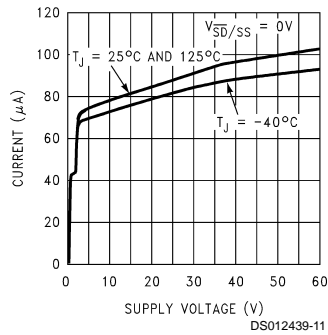
Standby Quiescent Current
