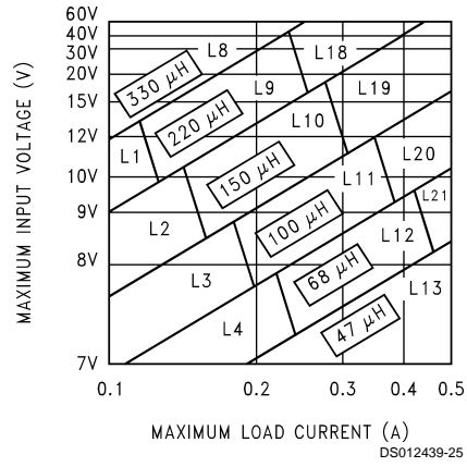
FIGURE 5. LM2594/LM2594HV-5.0
