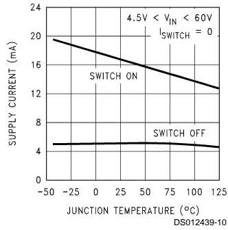
Quiescent Current
