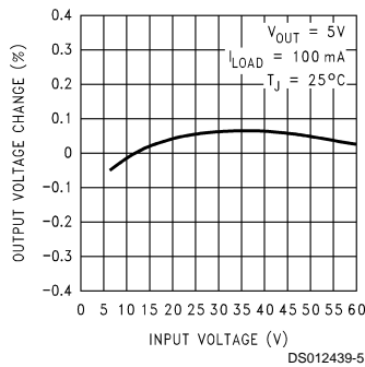
Line Regulation
