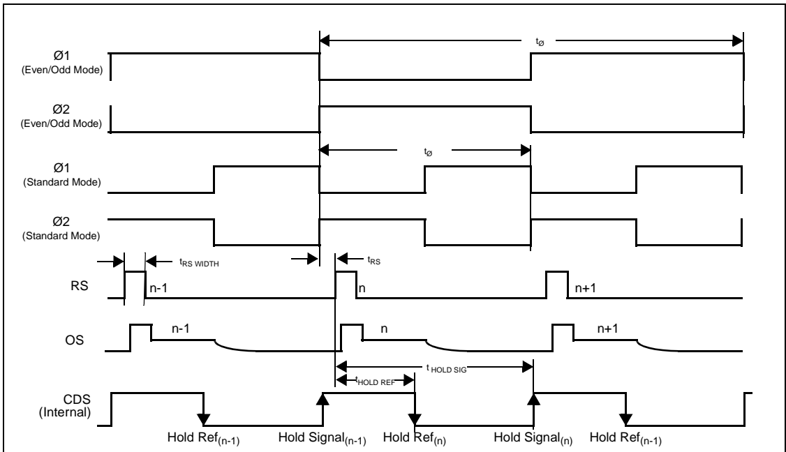
Diagram 12: CDS Timing
