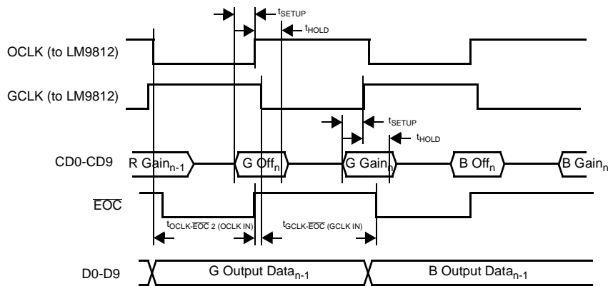
Diagram 19: Digital Data Timing, output data and coefficient data on separate buses, two clocks (OCLK and GCLK) for coefficient data, OCLK and GCLK input to LM9812, OCLK and GCLK phase = 180°, RD PIXEL held low.
