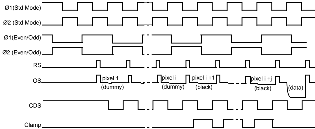
Diagram 13: Dummy Pixel and Optical Black Pixel Timing
