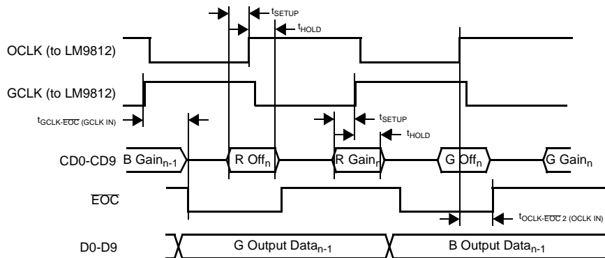
Diagram 18: Digital Data Timing, output data and coefficient data on separate buses, two clocks (OCLK and GCLK) for coefficient data, OCLK and GCLK input to LM9812, OCLK and GCLK phase = 0°, RD PIXEL held low.
