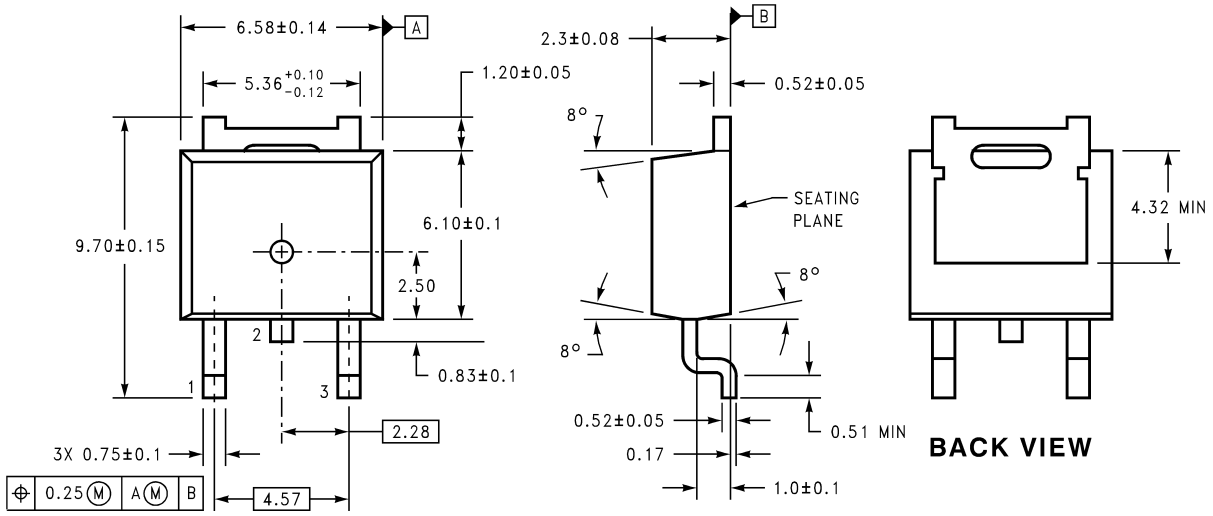
3-Lead TO-252 NS Package Number TD03B
