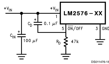
FIGURE 14. Delayed Startup
