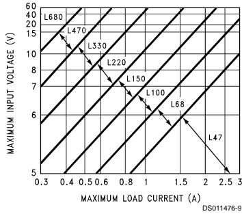
FIGURE 3. LM2576(HV)-3.3
