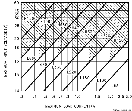
FIGURE 5. LM2576(HV)-12
