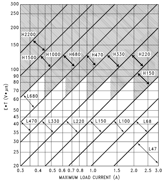
FIGURE 7. LM2576(HV)-ADJ
