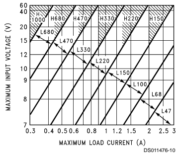
FIGURE 4. LM2576(HV)-5.0
