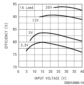
Efficiency
