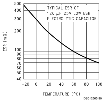
FIGURE 15. Capacitor ESR Change vs Temperature
