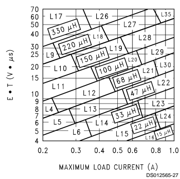
FIGURE 7. LM2595-ADJ
