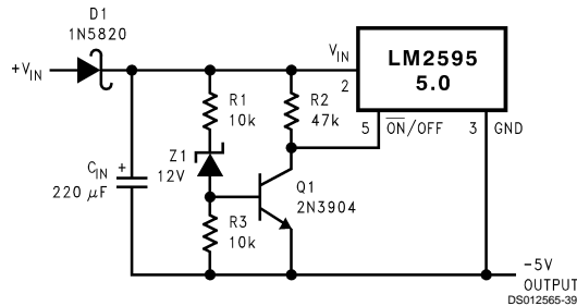
FIGURE 24. Undervoltage Lockout with Hysteresis for Inverting Regulator
