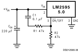
FIGURE 21. Delayed Startup
