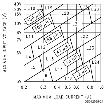
FIGURE 4. LM2595-3.3
