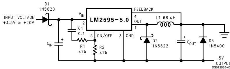
FIGURE 24. Undervoltage Lockout with Hysteresis for Inverting Regulator
