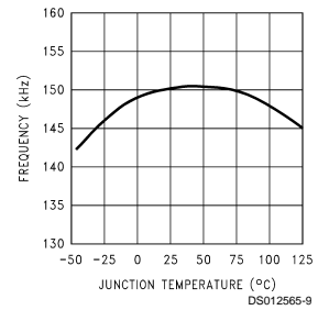
Switching Frequency
