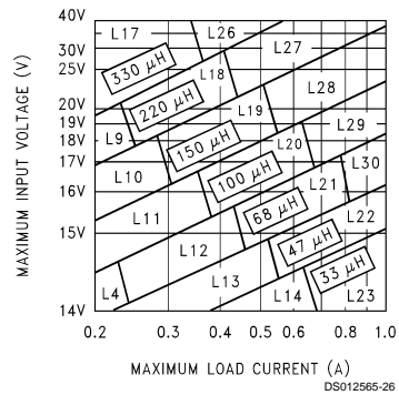
FIGURE 6. LM2595-12
