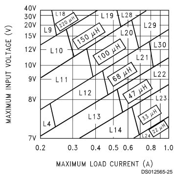
FIGURE 5. LM2595-5.0
