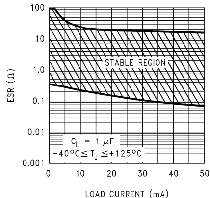
FIGURE 1. 1 \mu\text{F} ESR Range
