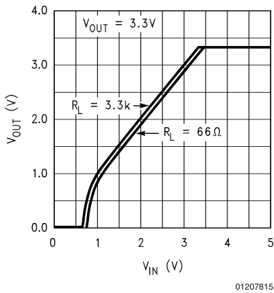
Dropout Characteristics
