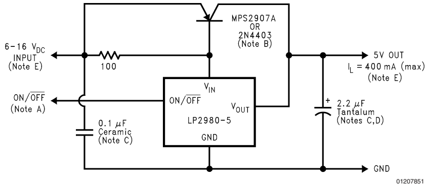
FIGURE 5. 5V/400mA Regulator
