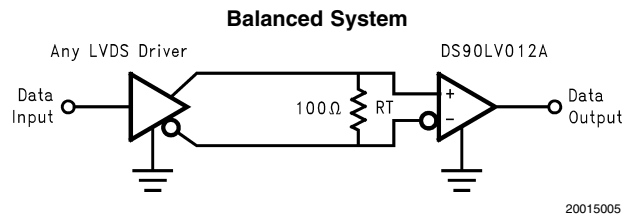
FIGURE 3. Point-to-Point Application (DS90LV012A)
