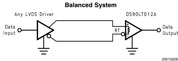
FIGURE 4. Point-to-Point Application (DS90LT012A)
