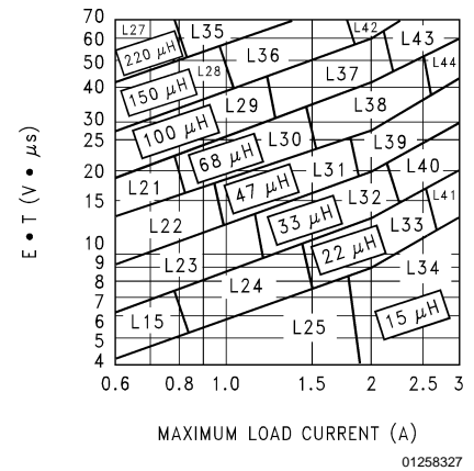
FIGURE 7. LM2596-ADJ
