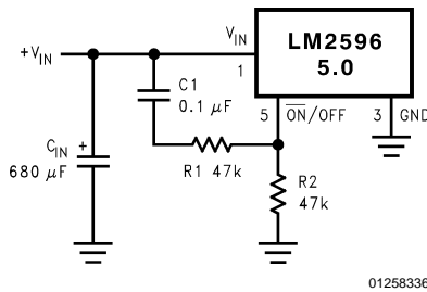
FIGURE 21. Delayed Startup
