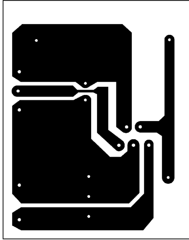
Copper Side
