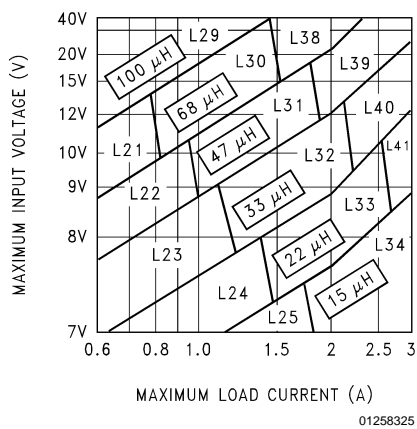
FIGURE 5. LM2596-5.0
