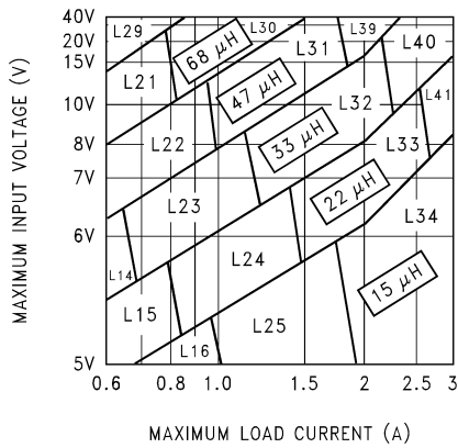
FIGURE 4. LM2596-3.3
