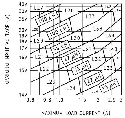
FIGURE 6. LM2596-12
