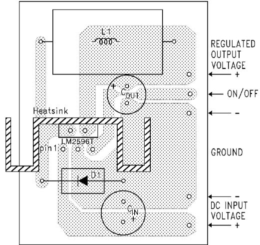
Component Side
