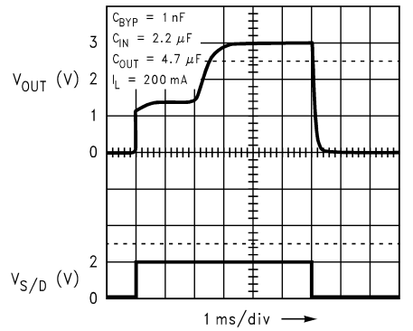
Turn-On Time (LP2988)
