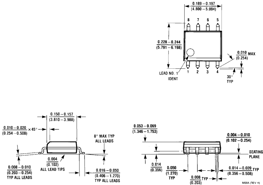
Order Number LM4809MA NS Package Number M08A
