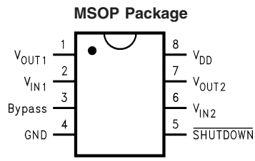
Top View Order Number LM4809MM See NS Package Number MUA08A
