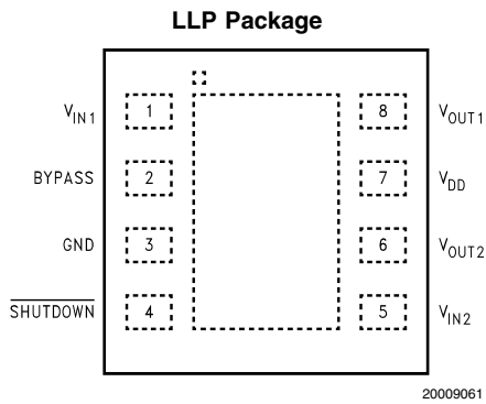
Top View Order Number LM4809LD See NS Package Number LDA08B
