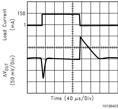
Load Transient Response ( V_{IN} = 3.2V )
