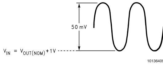
FIGURE 2. PSRR Input Test Signal
