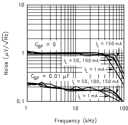
Output Noise Spectral Density
