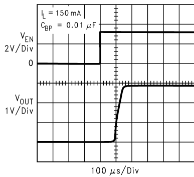
Enable Response ( V_{IN} = V_{OUT} + 0.2V )
