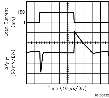
Load Transient Response ( V_{IN} = 4.2V )
