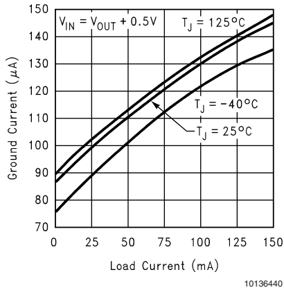
Ground Current vs Load Current
