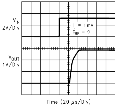
Start Up Time ( V_{IN} = V_{OUT} + 0.2V )
