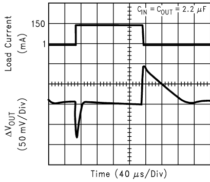
Load Transient Response ( V_{IN} = 3.2V )
