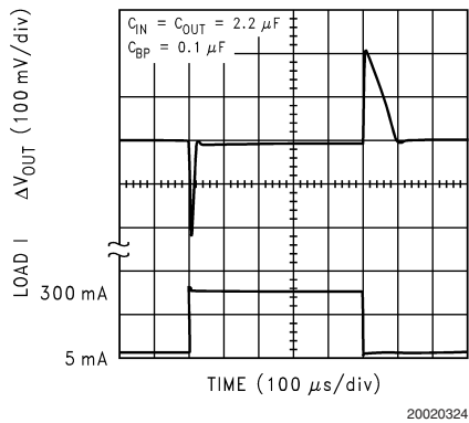
Load Transient Response ( V_{IN} = 3.5V )
