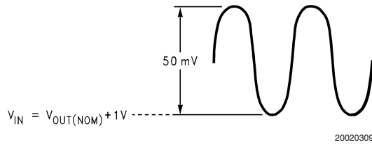
FIGURE 2. PSRR Input Perturbation
