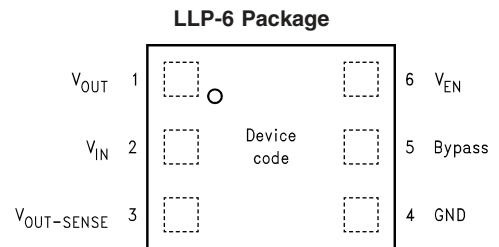
Top View See NS Package Number LDC06D
