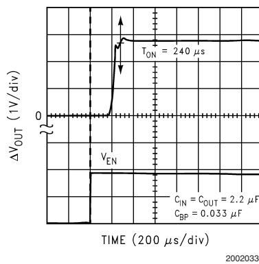
Enable Response ( T_{ON} )
