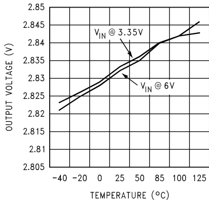
Output Voltage vs. Temperature ( V_{OUT} = 2.83V )
