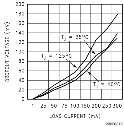
Dropout Voltage vs. Temperature ( V_{OUT} = 2.85V )
