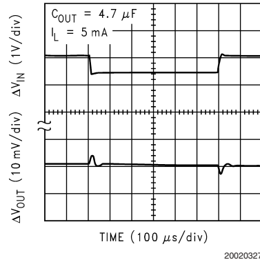
Line Transient Response ( V_{IN} = V_{OUT} + 1\text{V} to V_{OUT} + 1.6\text{V} )
