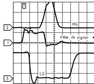
FIGURE 3. When Input Goes Low
