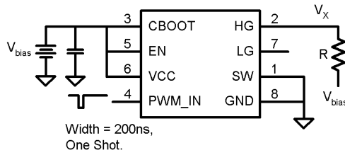
Test Circuit 2
