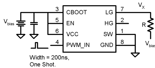
Test Circuit 4
