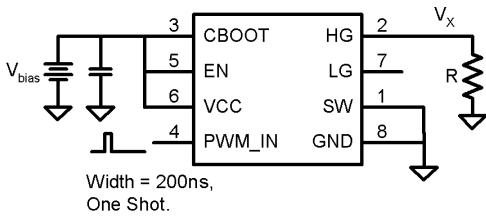
Test Circuit 1
