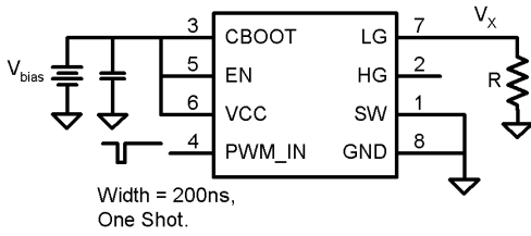
Test Circuit 3
