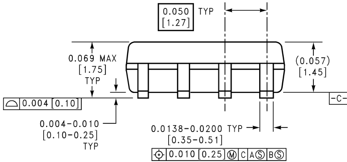
8-Lead Small Outline Package NS Package Number M08A
