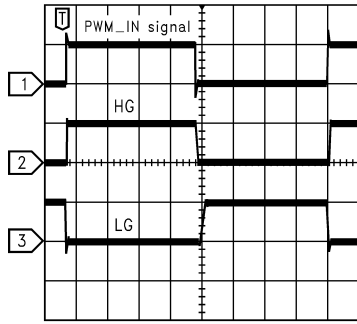
FIGURE 1. Switching Waveforms of Test Circuit
