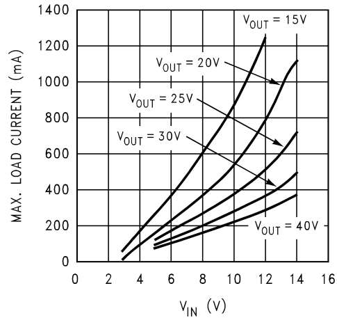
Max. Load Current vs VIN - "X"
