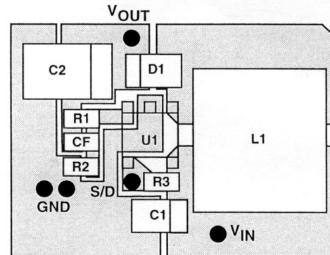
Recommended PCB Component Layout
