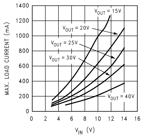
Max. Load Current vs VIN - "Y"
