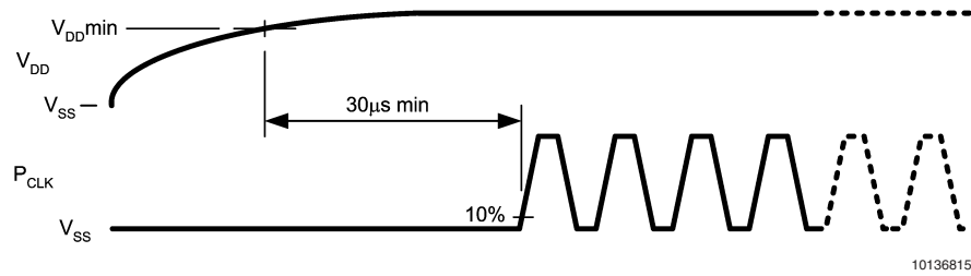
FIGURE 4. Power-On Reset Sequence
