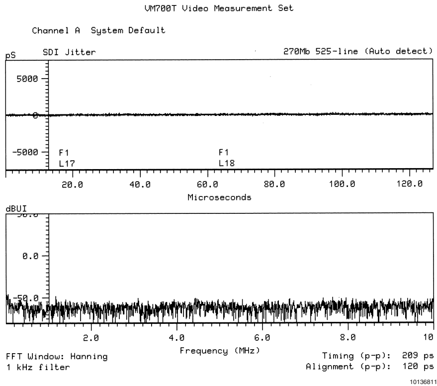
FIGURE 12. Jitter Plots
