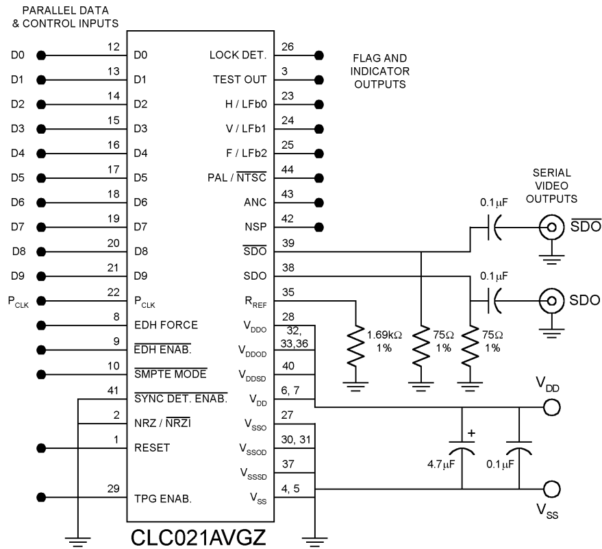
FIGURE 2. Test Circuit
