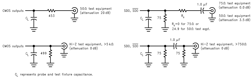
FIGURE 1. Test Loads
