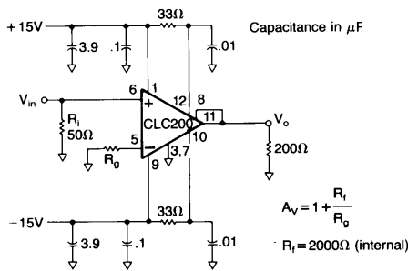
Figure 1: suggested non-inverting gain circuit
