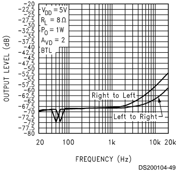
Crosstalk
