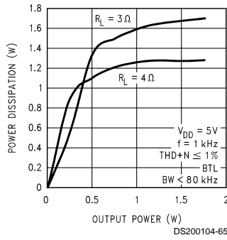
LM4840MH, LM4840LQ Power Dissipation vs Output Power
