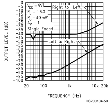
Crosstalk
