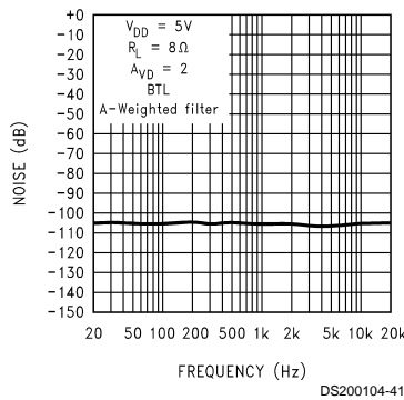
Noise Floor
