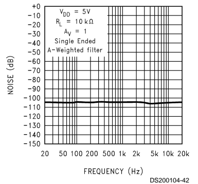
Noise Floor
