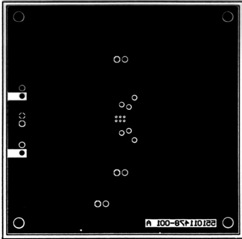
FIGURE 6. Recommended LQ PC board layout: bottom-side layout
