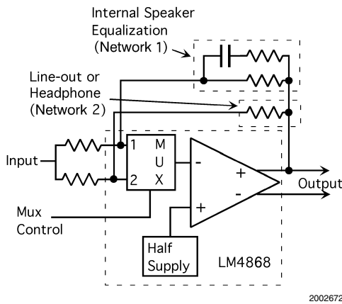
FIGURE 5. Input MUX Example
