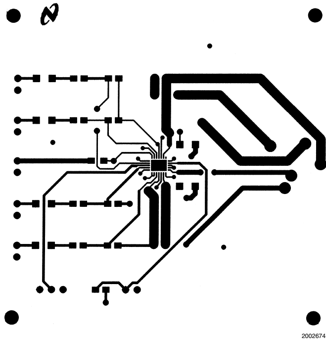
FIGURE 10. Recommended LQ PC Board Layout: Component-Side Layout
