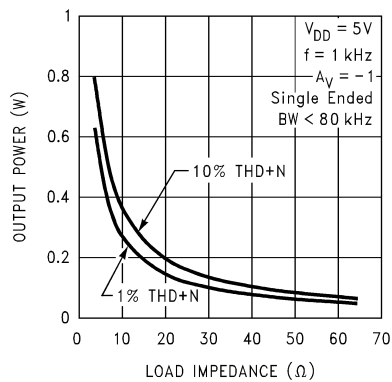
Output Power vs Load Impedance
