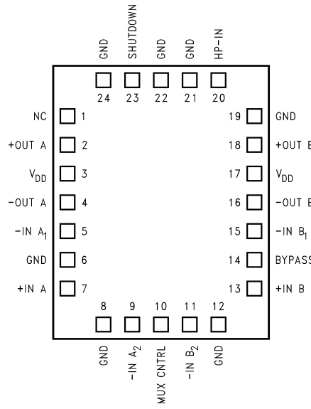
Top View Order Number LM4868LQ See NS Package Number LQA24A for Exposed-DAP LLP
