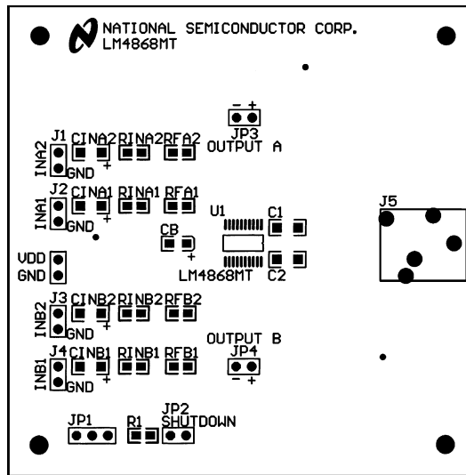
FIGURE 19. Recommended MT PC Board Layout: Component-Side Silkscreen
