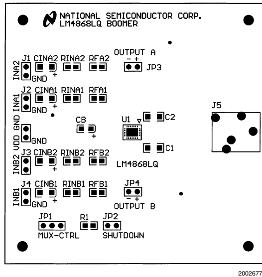
FIGURE 9. Recommended LQ PC Board Layout: Component-Side Silkscreen
