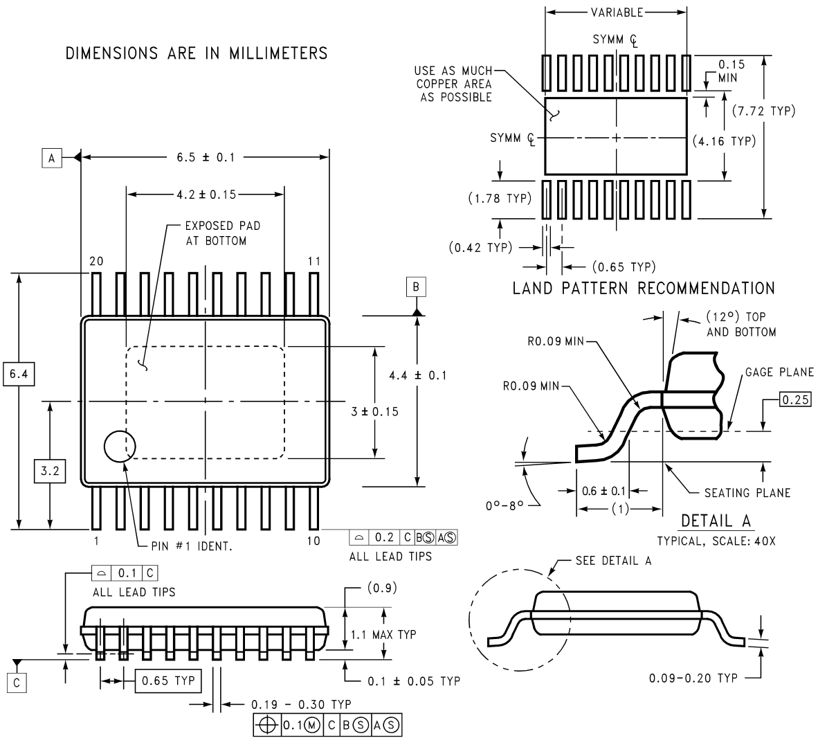
20-Lead MOLDED TSSOP, EXPOSED PAD, 6.5x4.4x0.9mm Order Number LM4868MTE NS Package Number MXA20A
