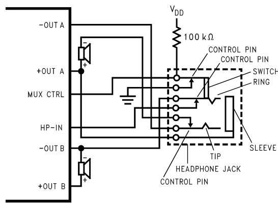
FIGURE 6. As configured, connecting headphones to this jack automatically selects the stereo headphone amplifier and, with the additional NC switch, changes MUX channels (Network 2 in Figure 5)
