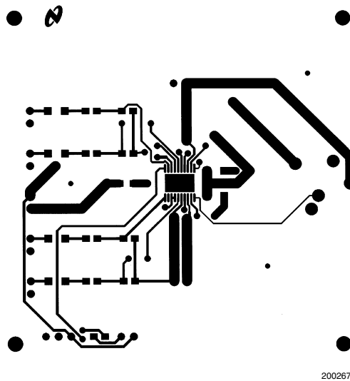
FIGURE 15. Recommended MTE PC Board Layout: Component-Side Layout
