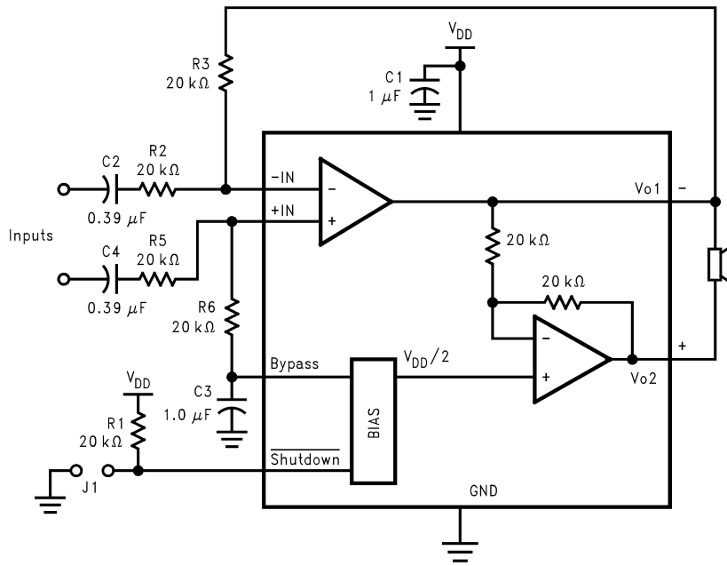
DIFFERENTIAL AMPLIFIER CONFIGURATION FOR LM4890
