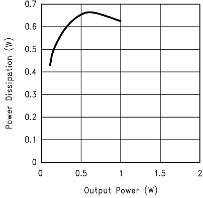
Power Dissipation vs Output Power V_{DD} = 5V, 1kHz, 8\Omega, THD \leq 1.0\%
