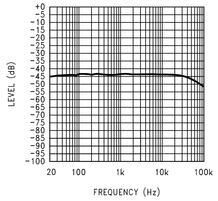
Power Supply Rejection Ratio (PSRR) @ A_V = 2 V_{DD} = 2.6V , V_{ripple} = 200mvp-p , R_L = 8\Omega , R_{IN} = 10\Omega
