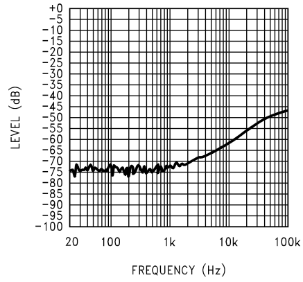
Power Supply Rejection Ratio (PSRR) @ A_V = 2 V_{DD} = 5V , V_{ripple} = 200mvp-p R_L = 8\Omega , R_{IN} = Float
