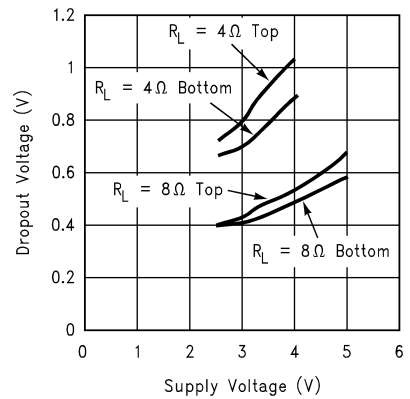
Clipping (Dropout) Voltage vs Supply Voltage
