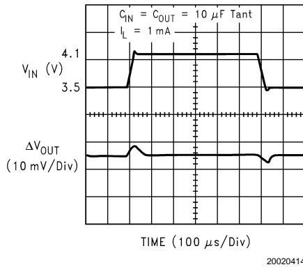
Line Transient Response (LP3984-3.1)
