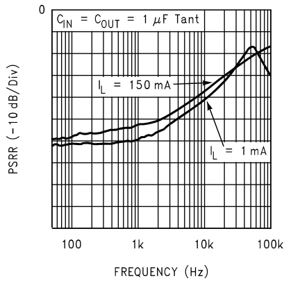
Power Supply Rejection Ratio ( V_{IN} = 3.5V )
