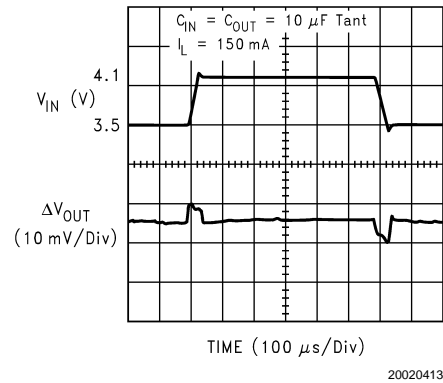
Line Transient Response (LP3984-3.1)
