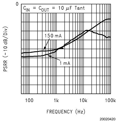
Power Supply Rejection Ratio ( V_{IN} = 3.5V )
