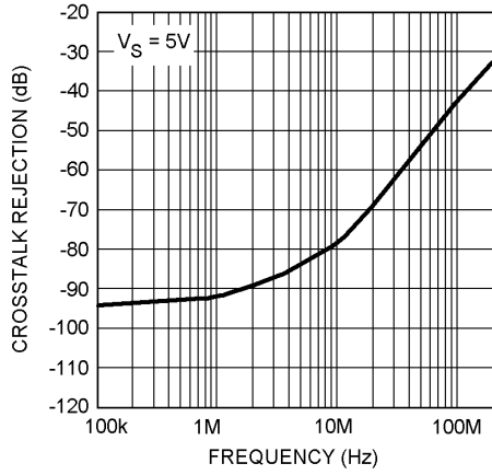
CrossTalk vs. Frequency (LMH6655 only)
