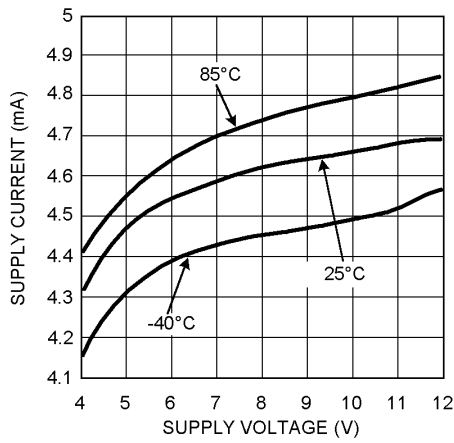
Supply Current per Channel vs. Supply Voltage
