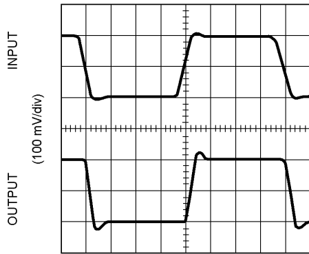
Non-Inverting Small Signal Pulse Response ( V_S = 5\text{V} )
