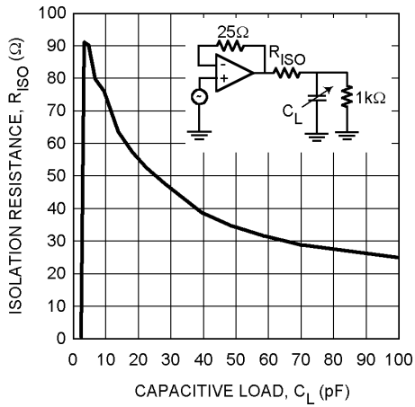
Isolation Resistance vs. Capacitive Load
