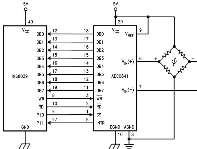
ADC0841_INS8039 Interface
