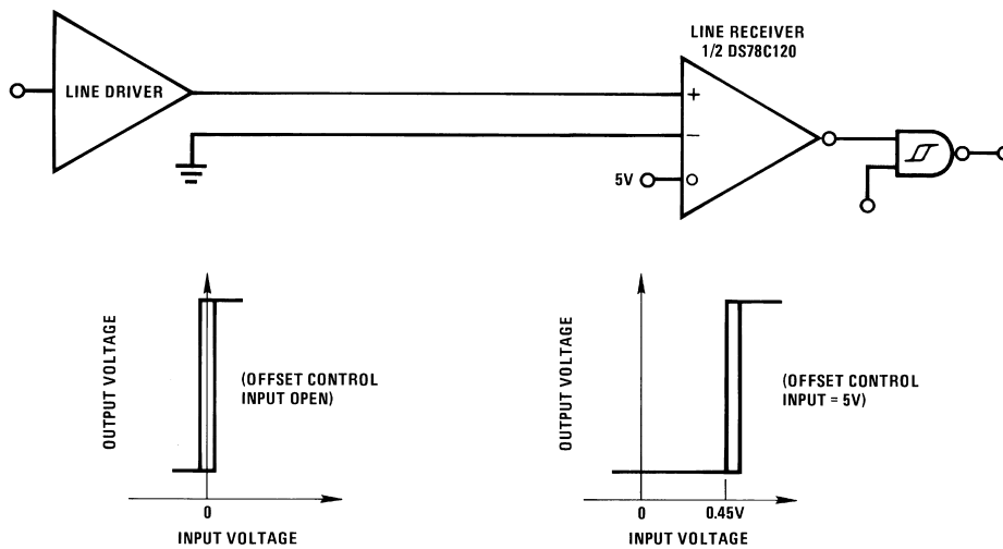
Unbalanced RS-423 and RS-232 Fail-Safe
