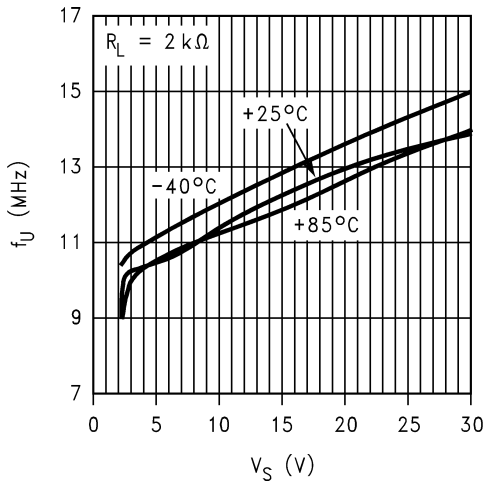
Unity Gain Frequency vs. V_S
