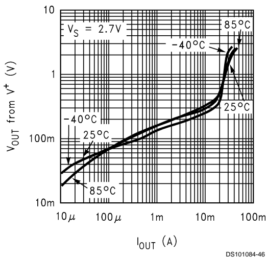
Output Voltage vs. Output Sourcing Current
