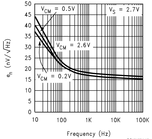
Input Noise Voltage for Various V_{CM}
