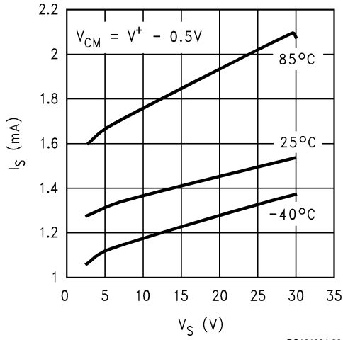
I_S vs. V_S (NPN side)
