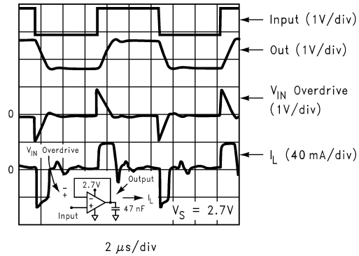
FIGURE 5. Buffer Amplifier scope photo
