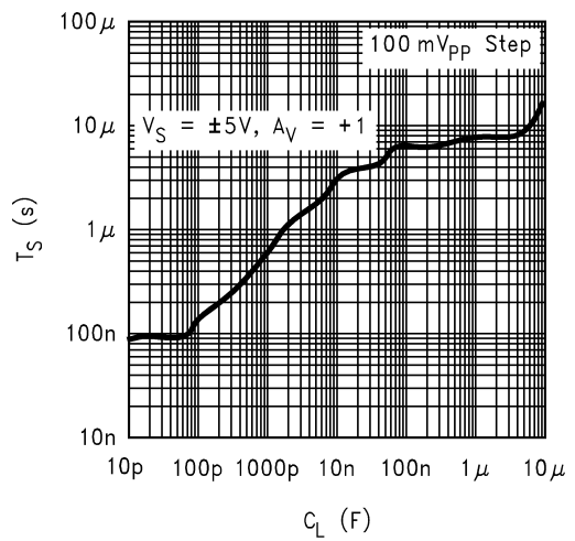
±5% Settling Time vs. Cap Load
