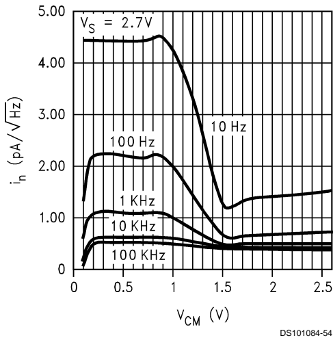
Input Noise Current vs. V_{CM}
