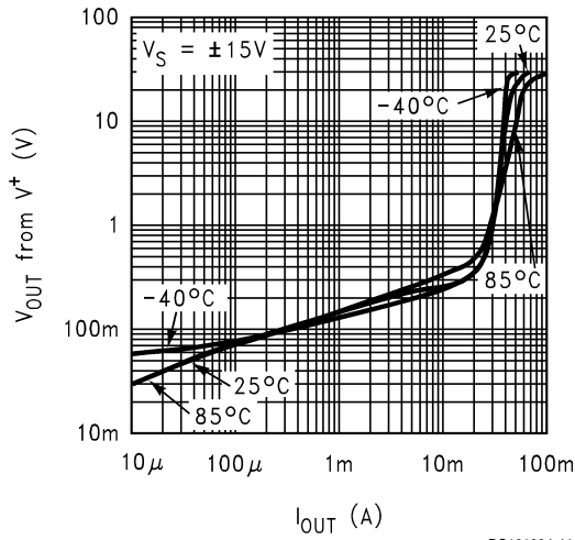
Output Voltage vs. Output Sourcing Current
