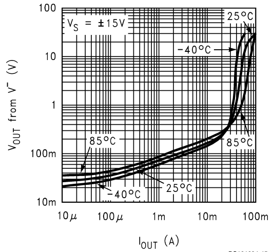
Output Voltage vs. Output Sinking Current
