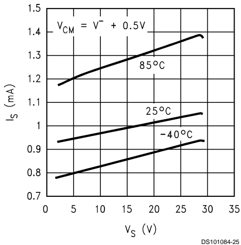
I_S vs. V_S (PNP side)
