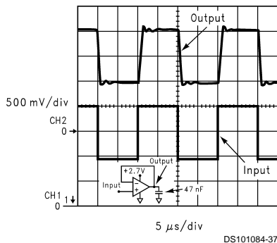
Output Response with Heavy Capacitive Load
