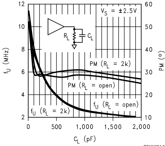
Unity Gain Freq. and Phase Margin vs. C_L
