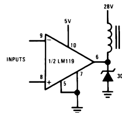
Relay Driver
