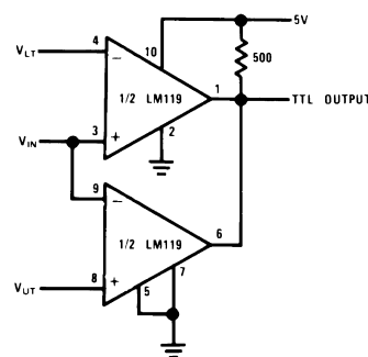
Window Detector
