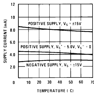
Supply Currents
