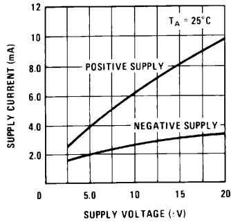
Supply Current
