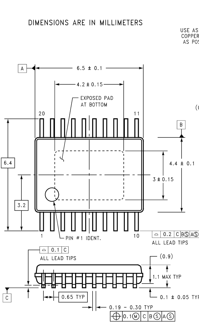
20-Lead Molded TSSOP, Exposed Pad, 6.5x4.4x0.9mm Order Number LM4863MTE NS Package Number MXA20A
