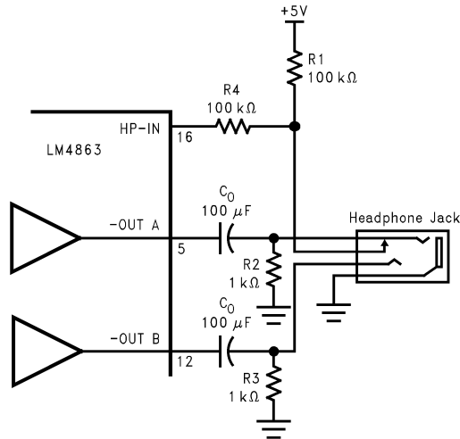
FIGURE 2. Headphone Circuit
