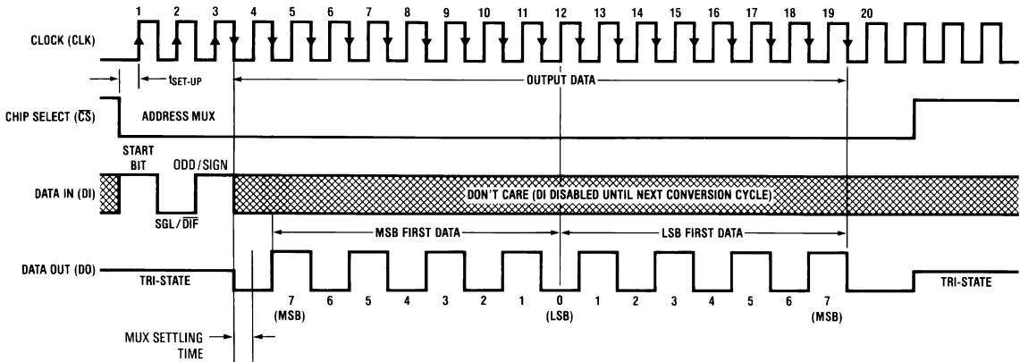
ADC0832 Timing
