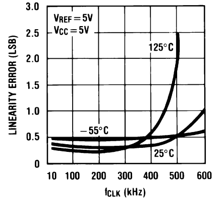
Linearity Error vs. f_{CLK}
