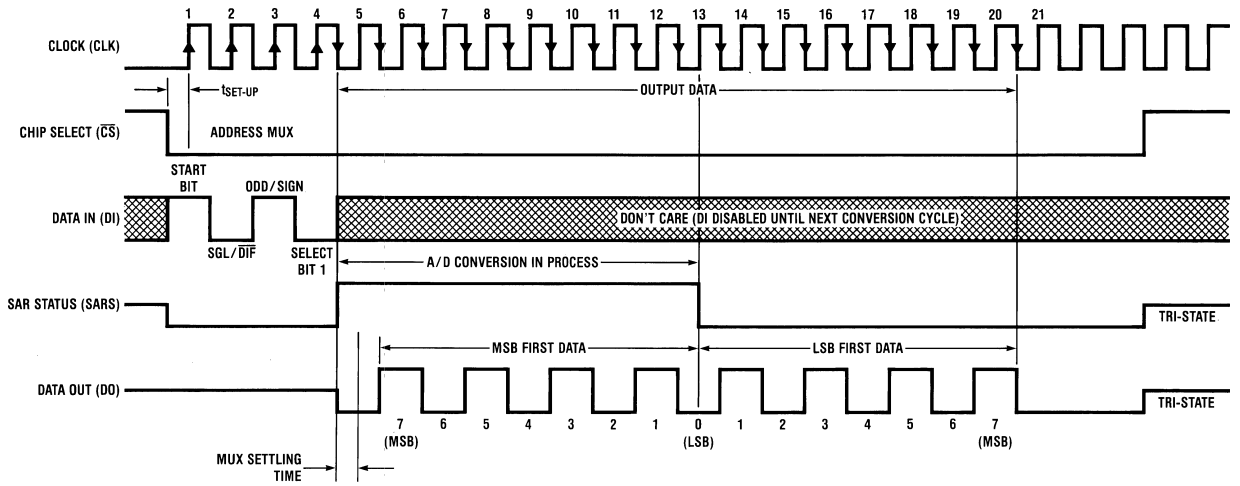
ADC0834 Timing
