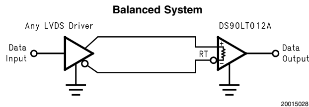
FIGURE 4. Point-to-Point Application (DS90LT012A)
