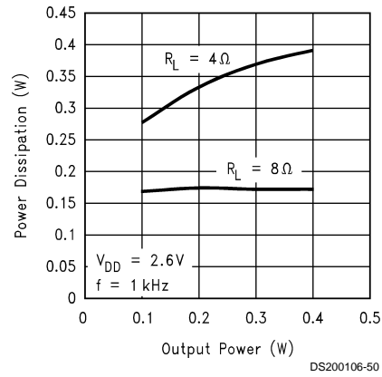
Power Dissipation vs Output Power V DD = 2.6V
