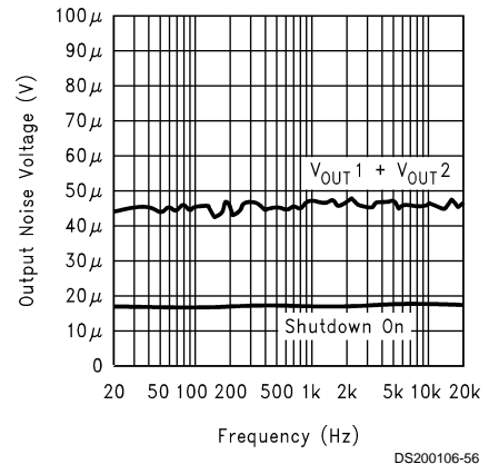
Noise Floor
