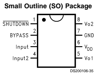
Top View Order Number LM4820M-6 See NS Package Number M08A
