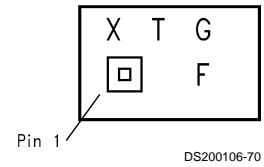
Top View X - Date Code T - Die Traceability G - Boomer Family F - LM4820IBP-6
