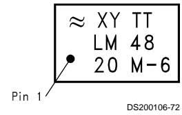
Top View XY - Date Code TT - Die Traceability Bottom 2 lines - Part Number ( LM4820M-6 )
