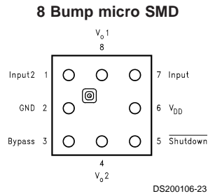
Top View Order Number LM4820IBP-6, LM4820IBPX-6 See NS Package Number BPA08DDB
