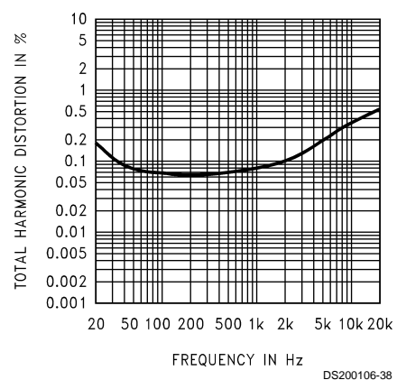
THD+N vs Frequency at V_{DD} = 3.3V, 8\Omega R_L , and PWR = 150mW
