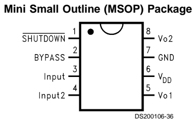
Top View Order Number LM4820MM-6 See NS Package Number MUA08A
